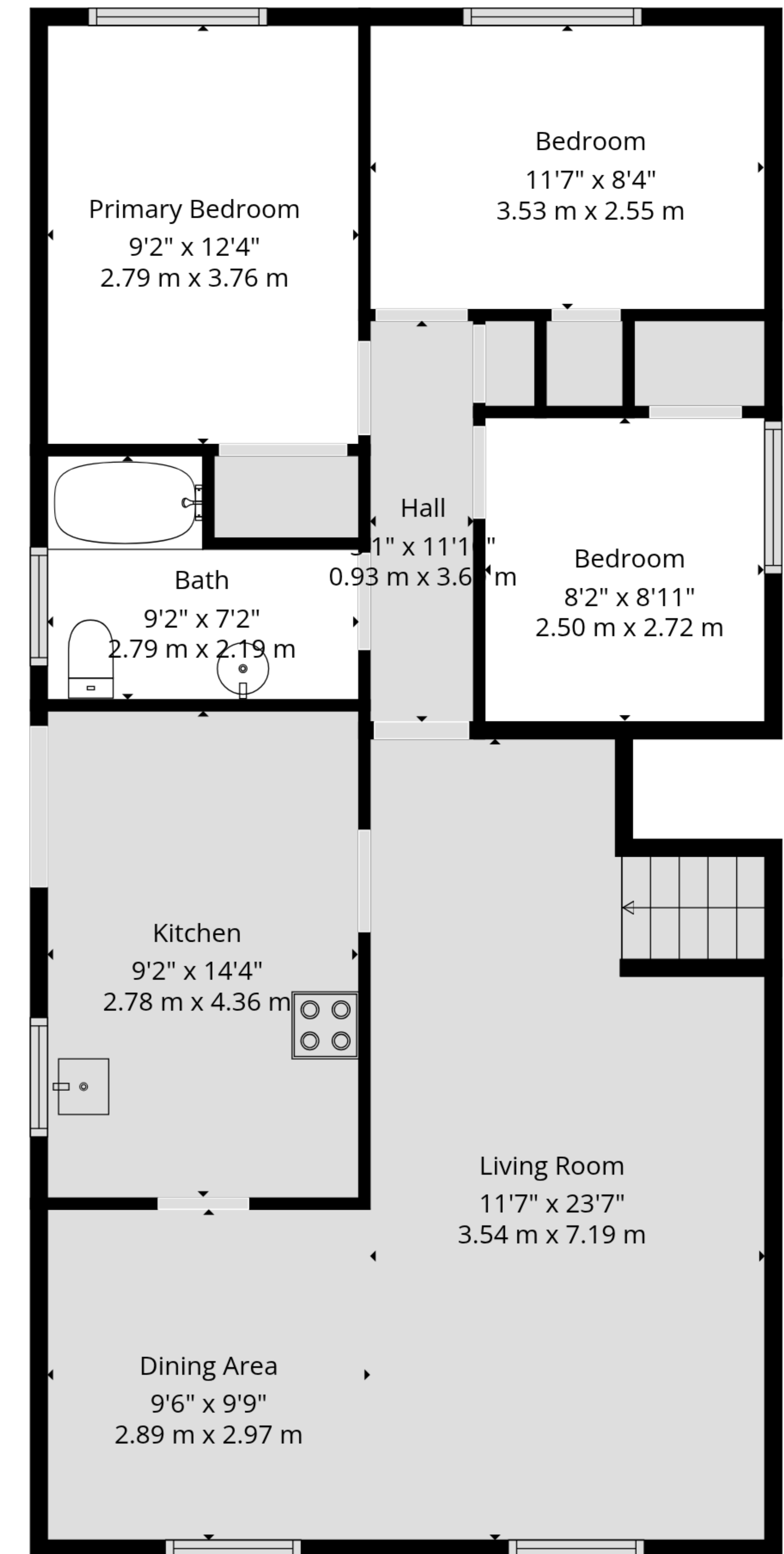
Main Floor
