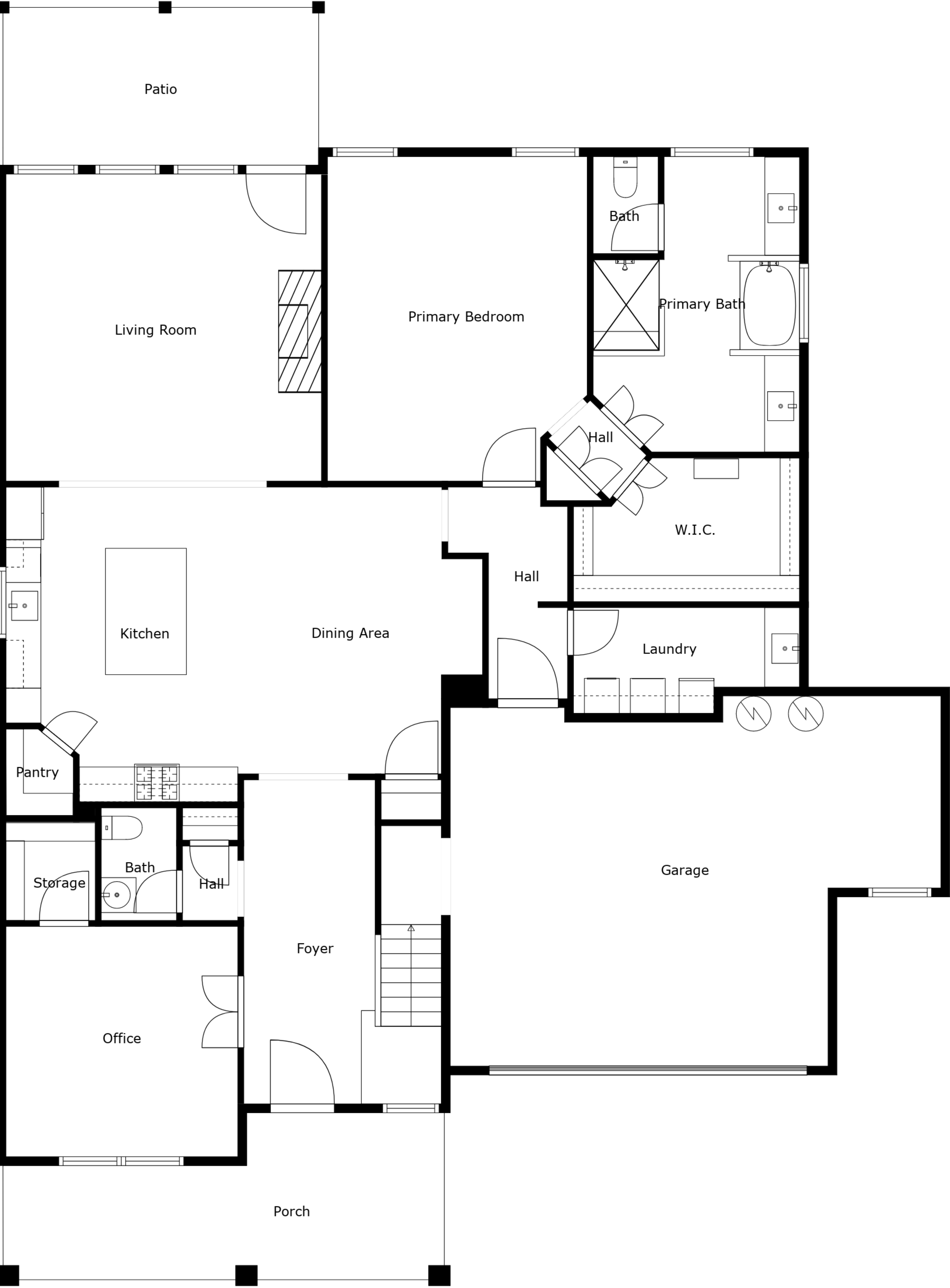
Floor 1
