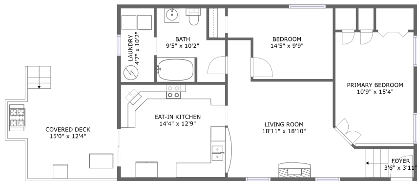
FLOOR 2
