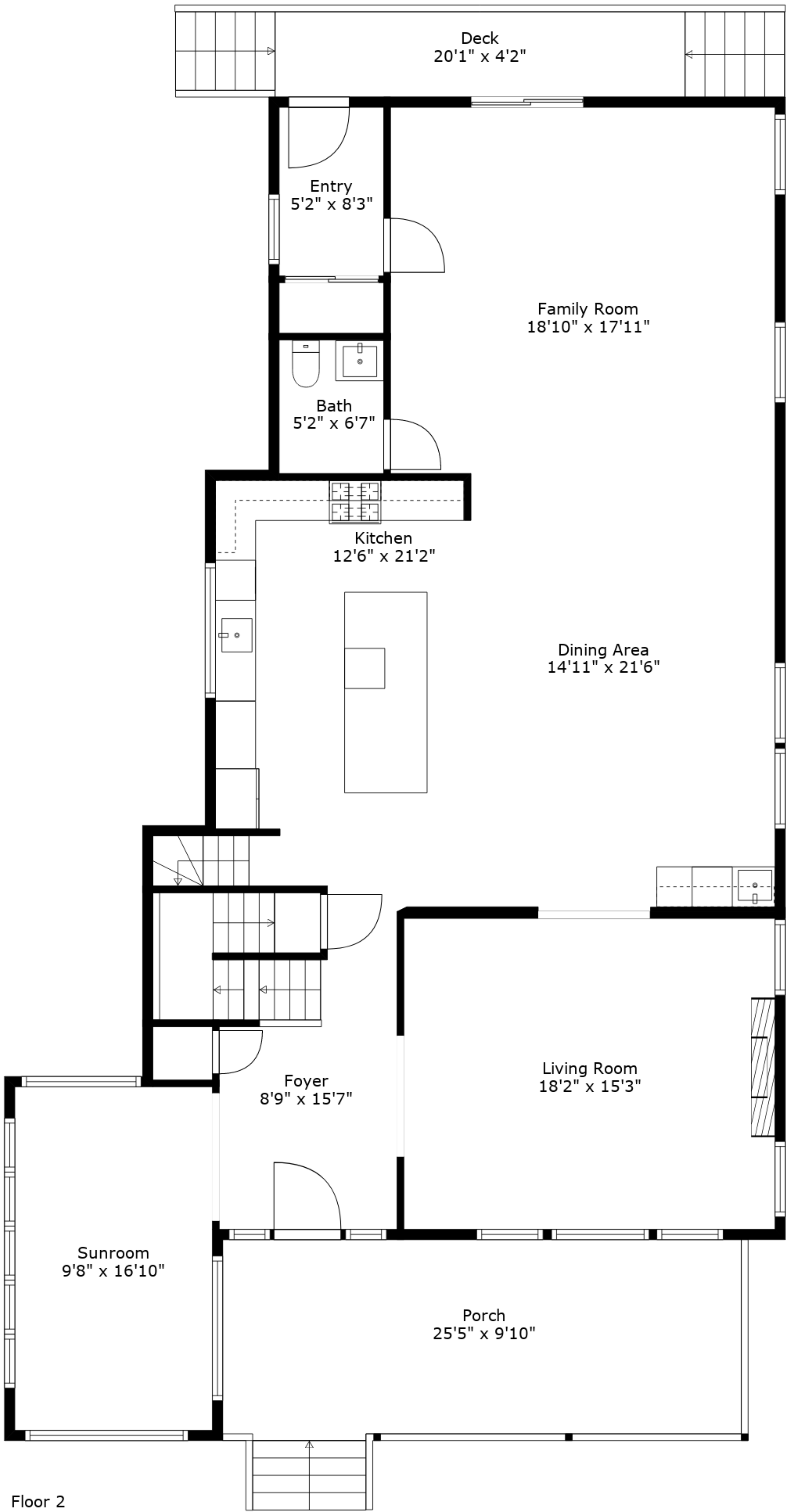
Floor 2
