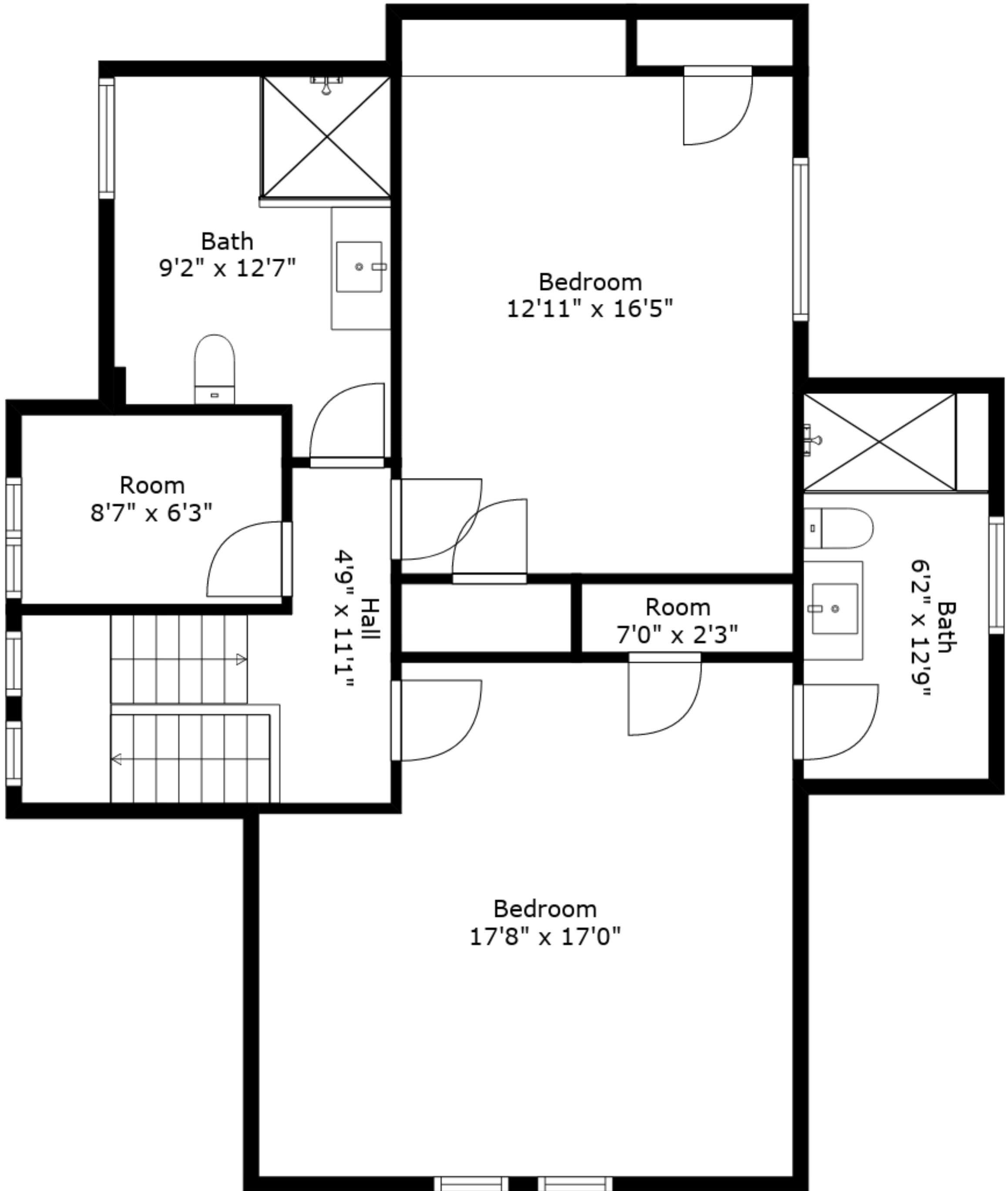
Floor 4
