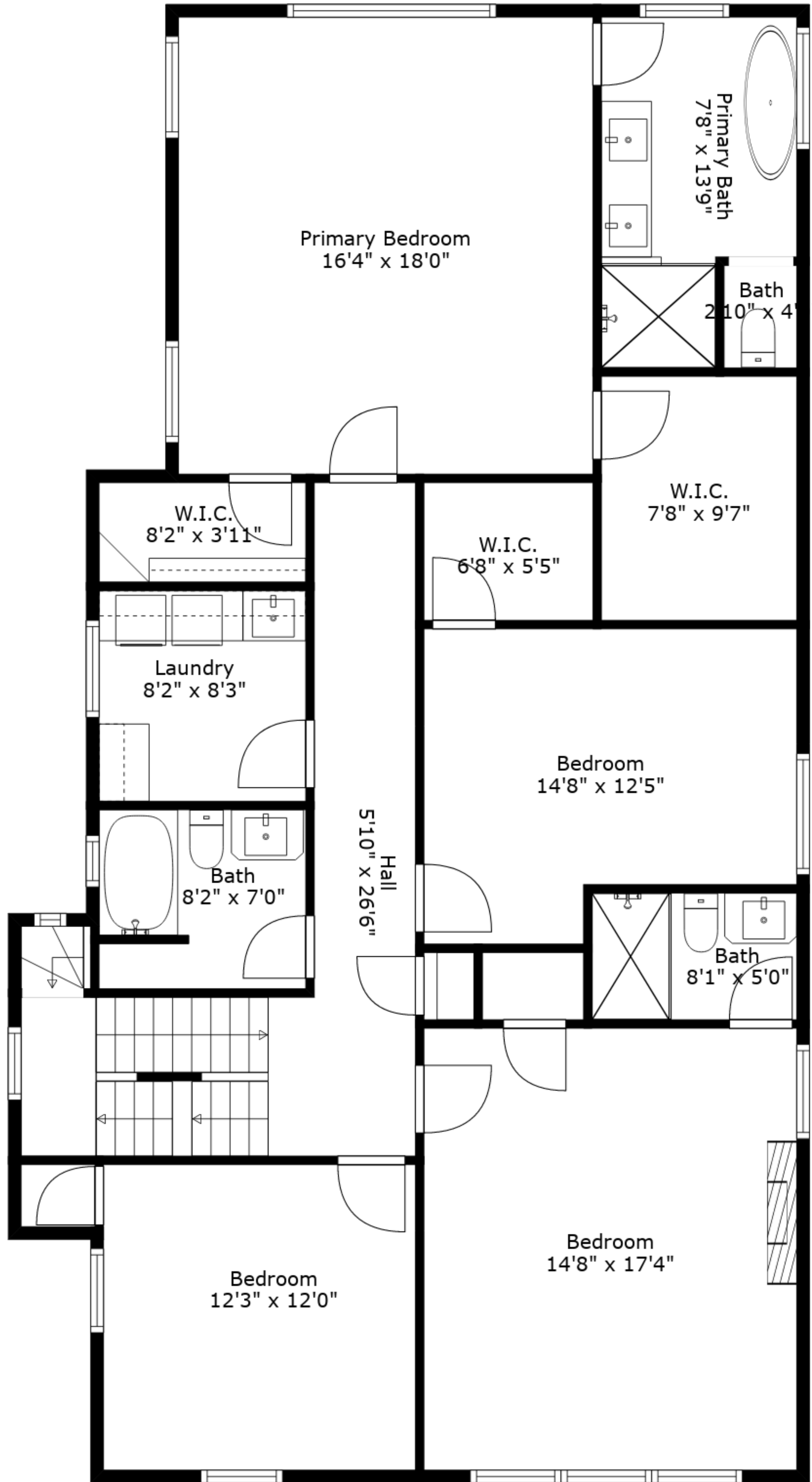
Floor 3
