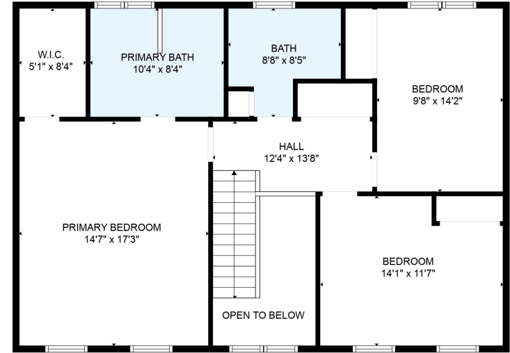
FLOOR 3
