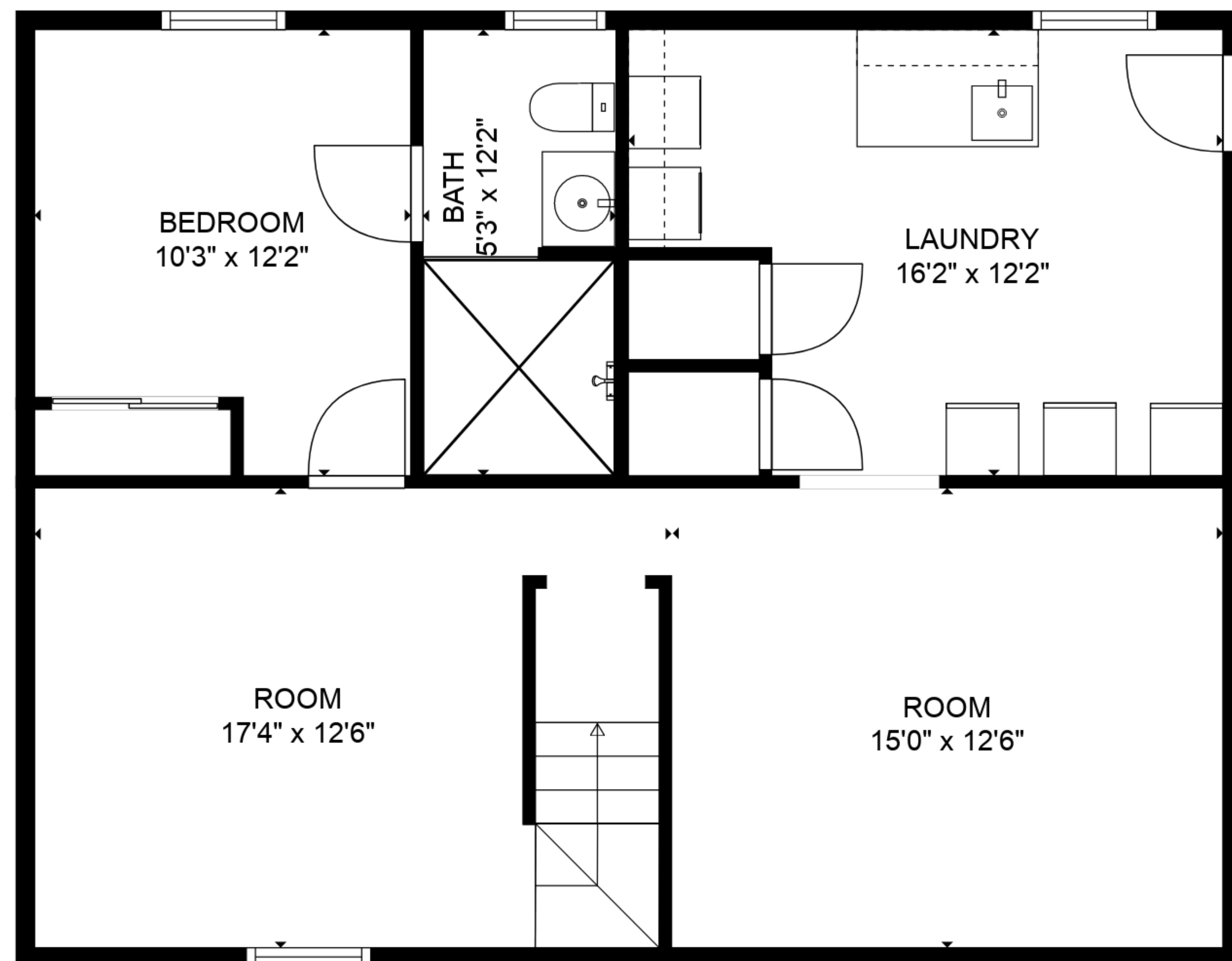
FLOOR 1
