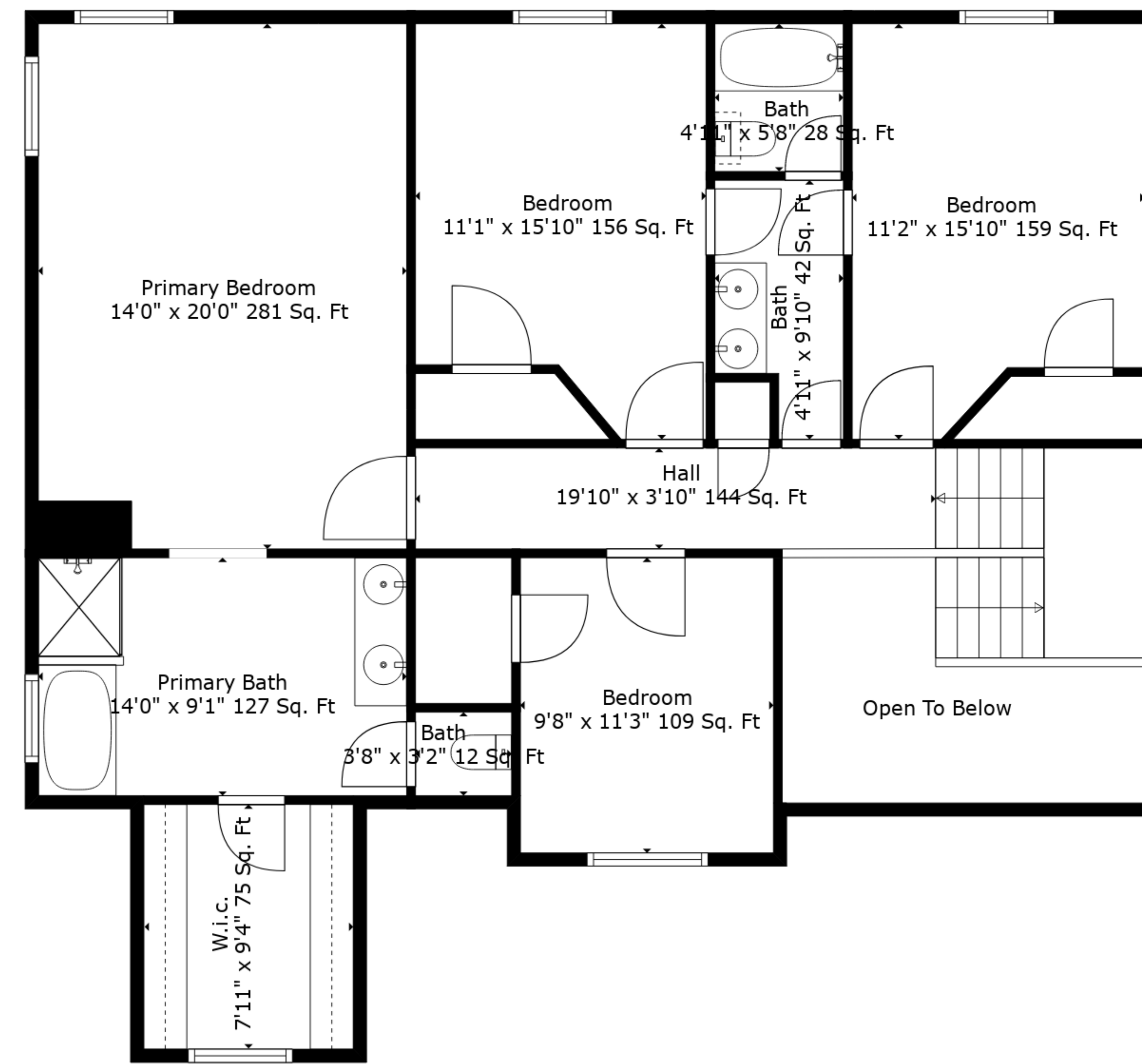
Floor 3
