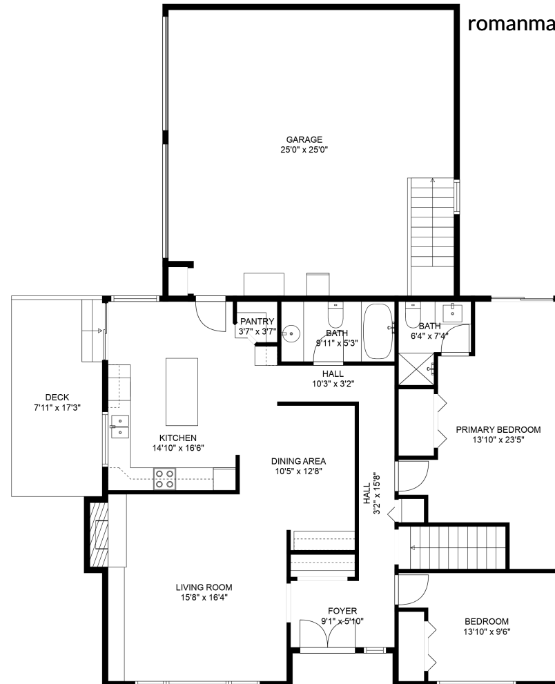
FLOOR 2
