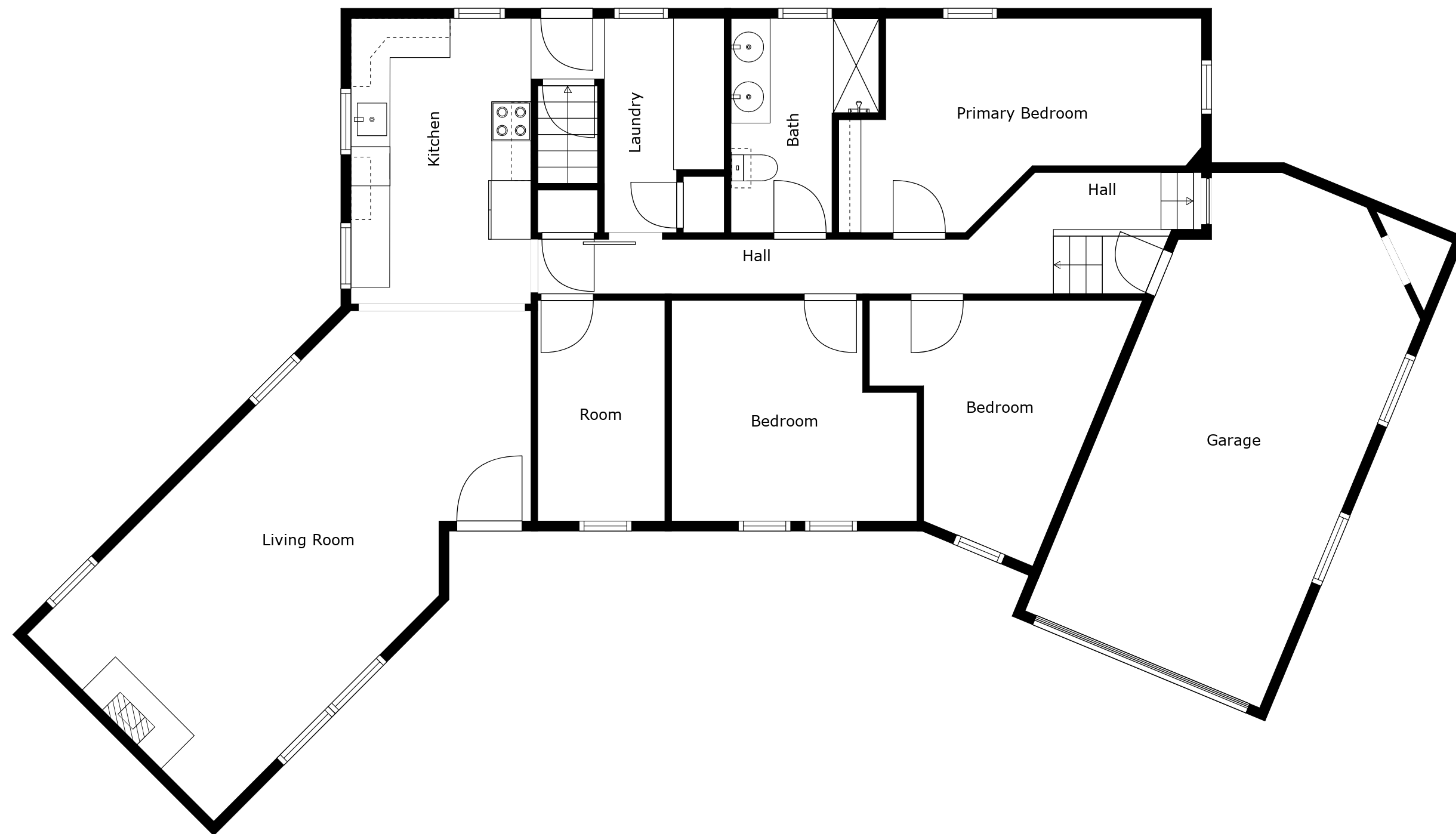
Floor 2
