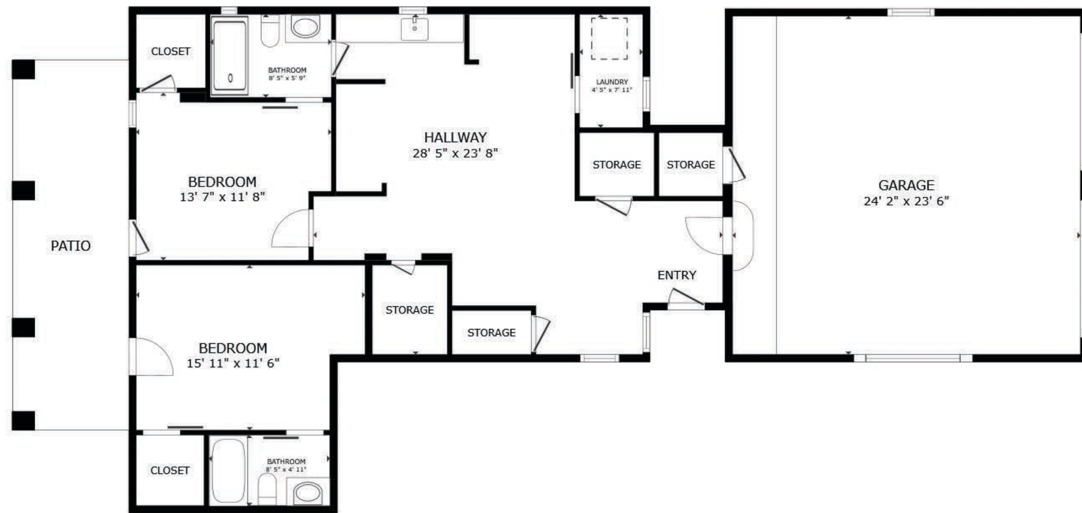
FLOOR 1
