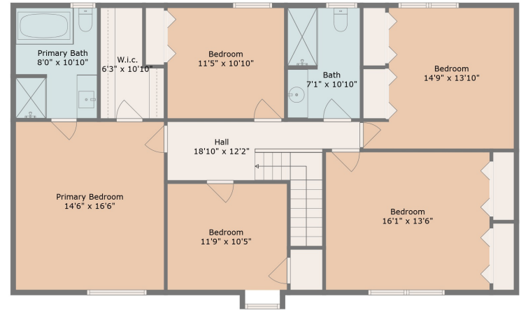
Floor 3
