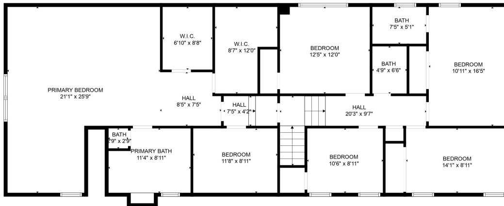
FLOOR 3
