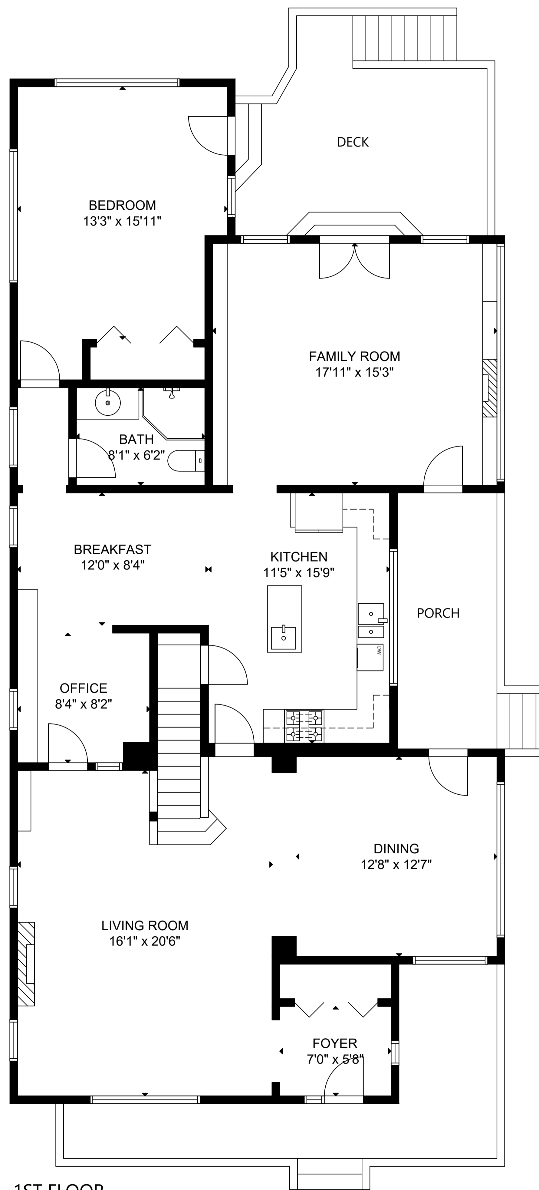
1ST FLOOR
