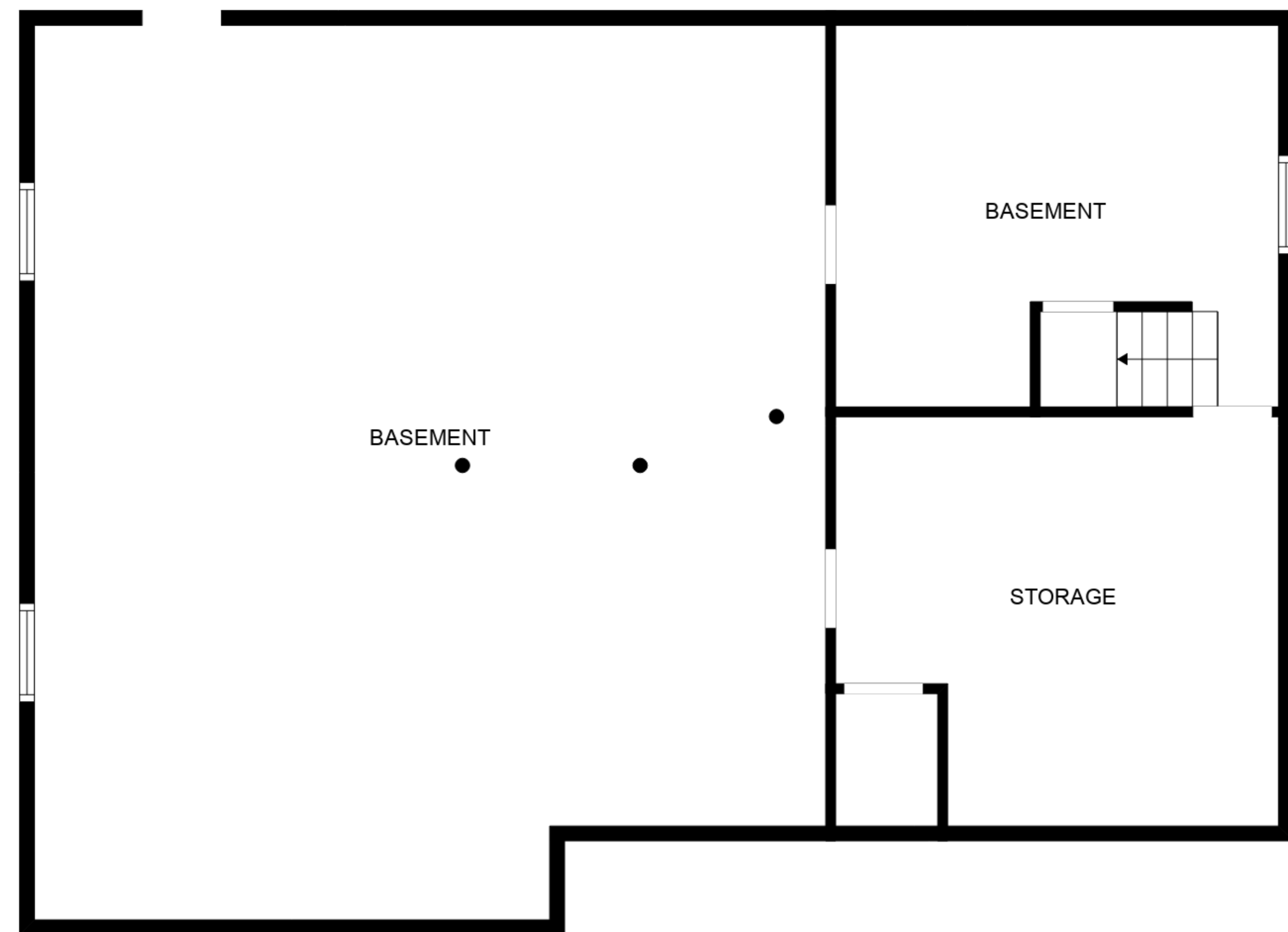
FLOOR 1
