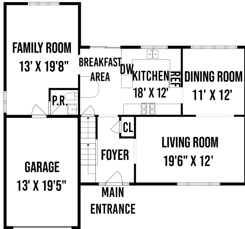
MAIN FLOOR
