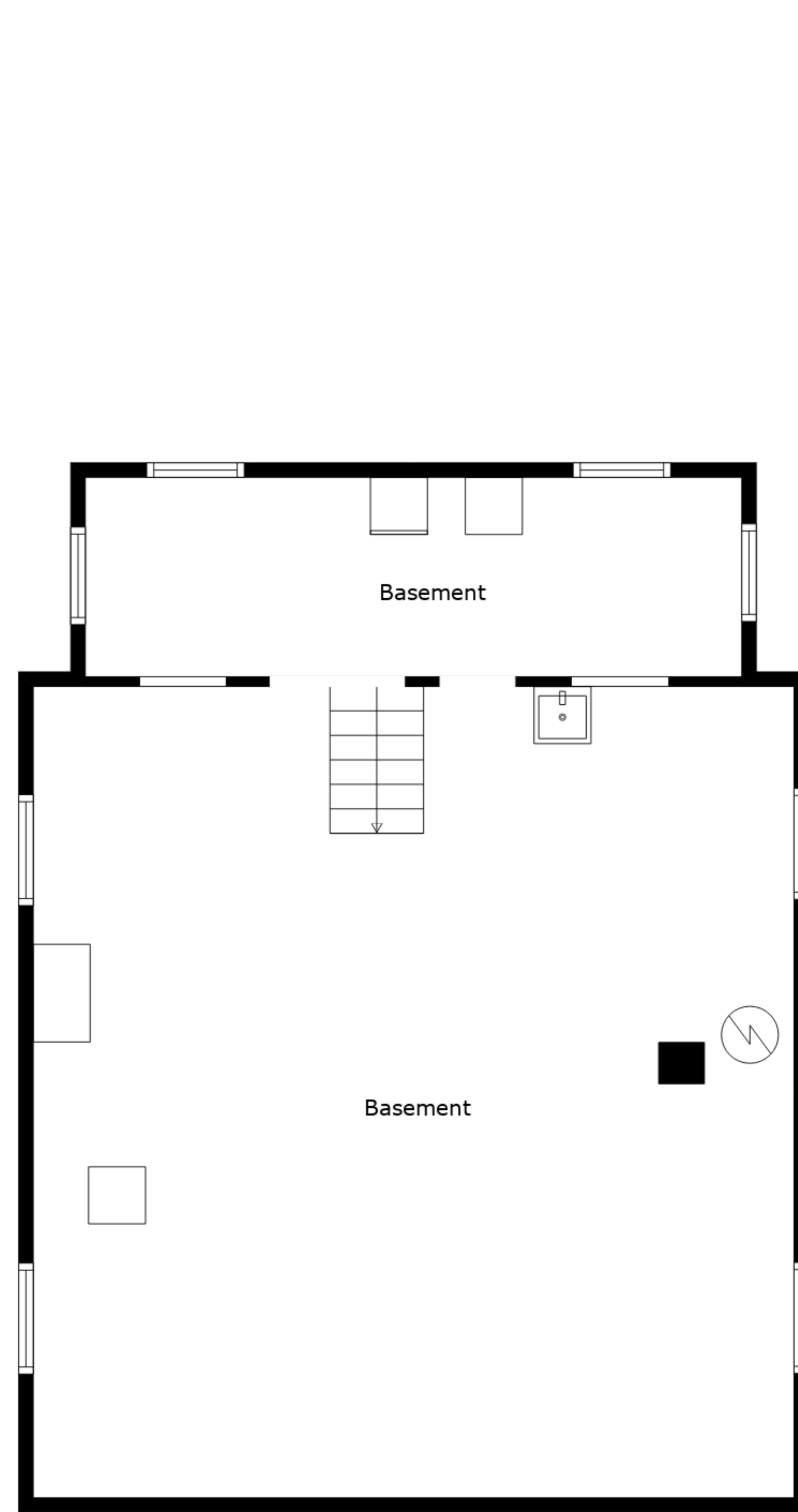
Floor 1
