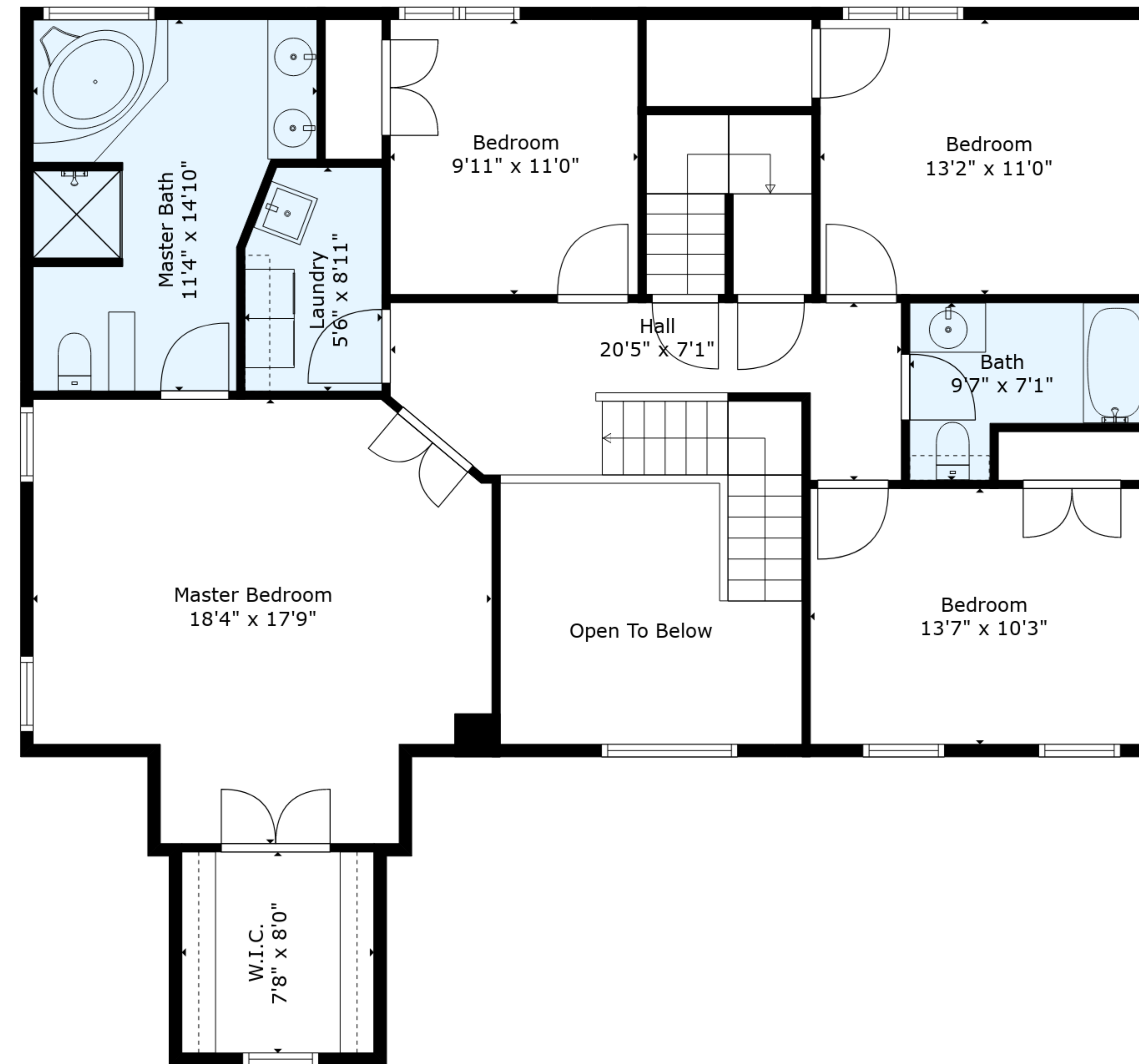
Floor 2
