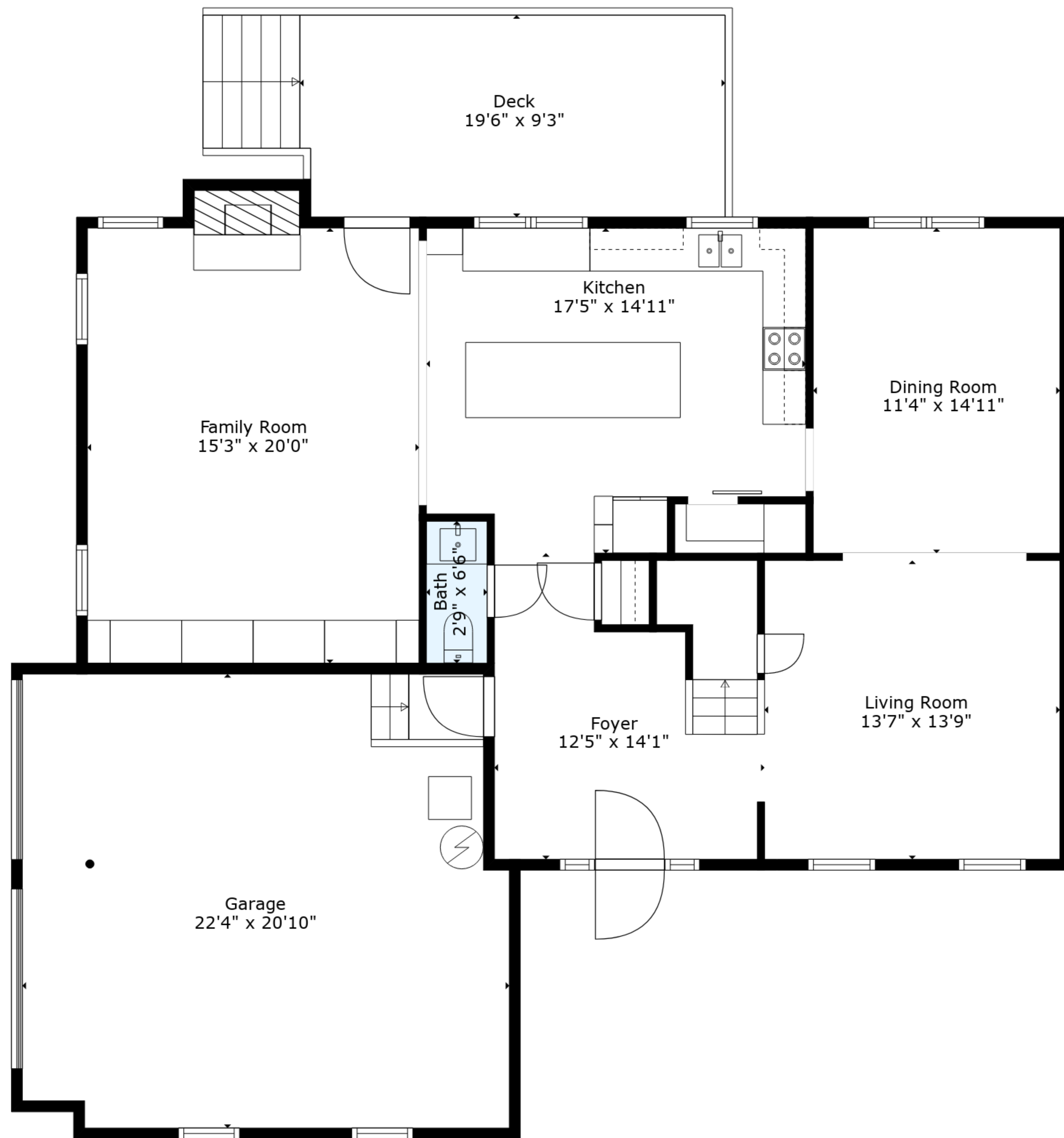
Floor 1
