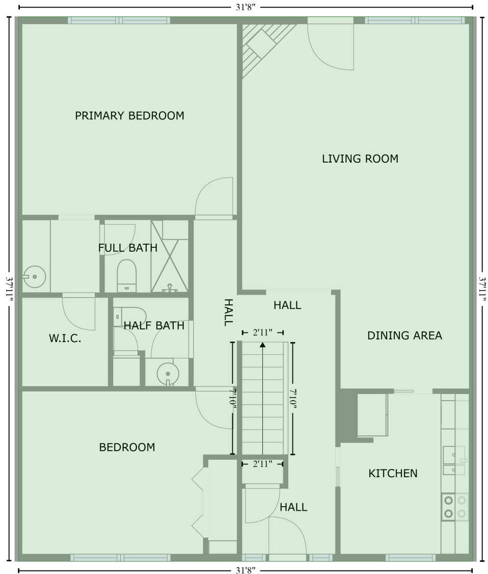
FLOOR 2 [AREA: 1201]
