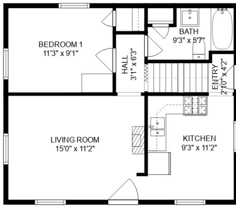
MAIN FLOOR
