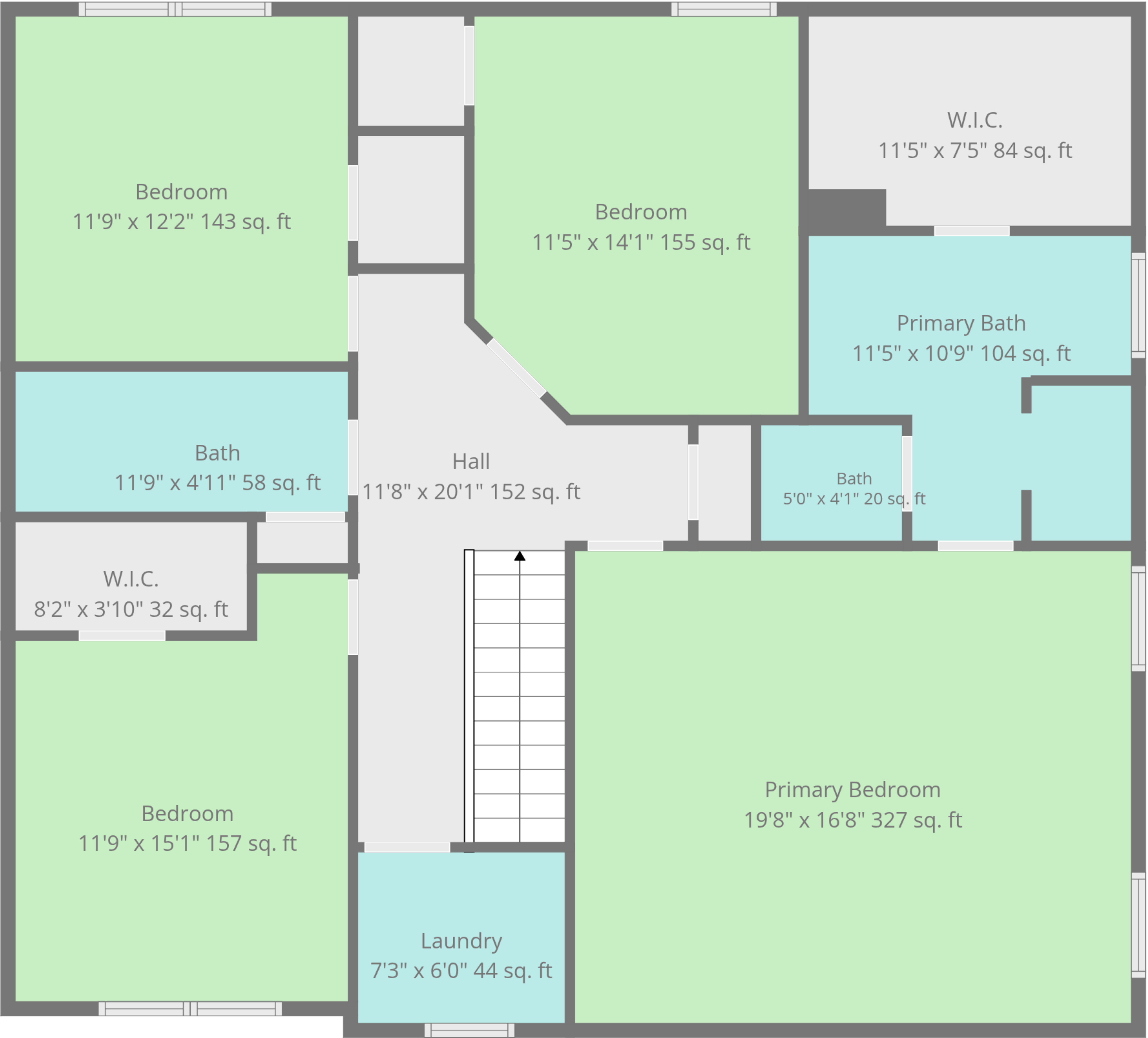
2nd Floor
