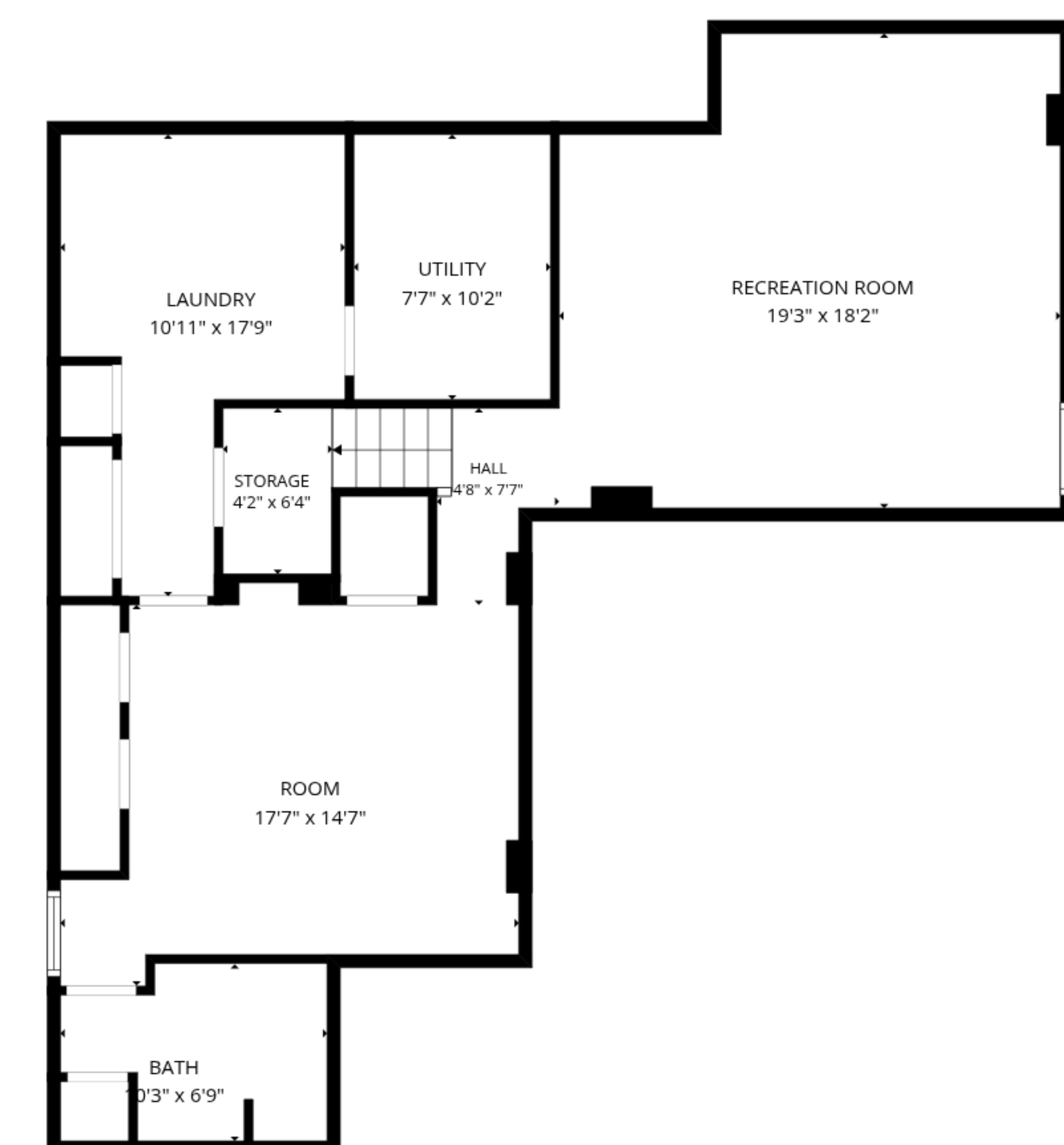
Basement
