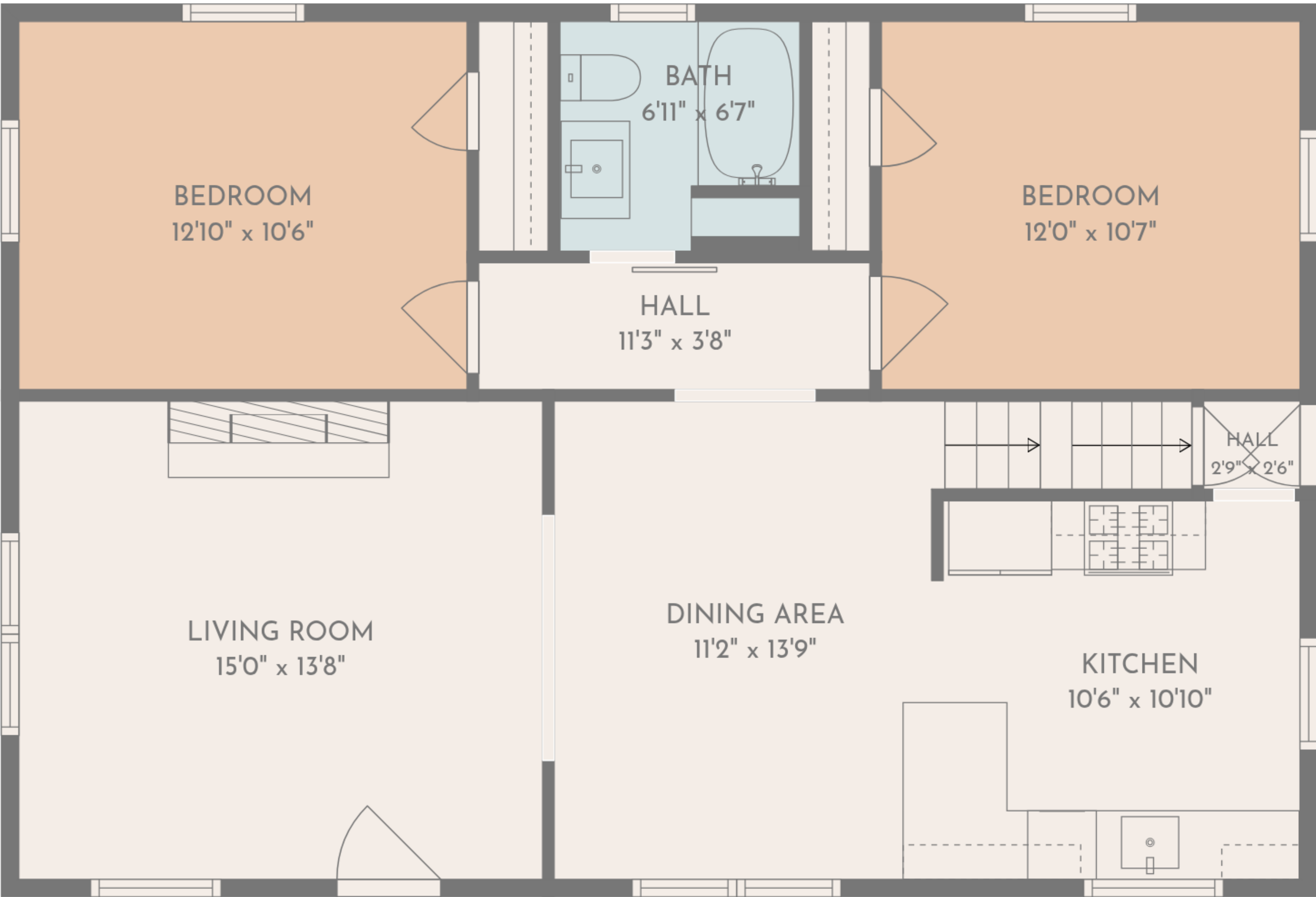
1st floor
