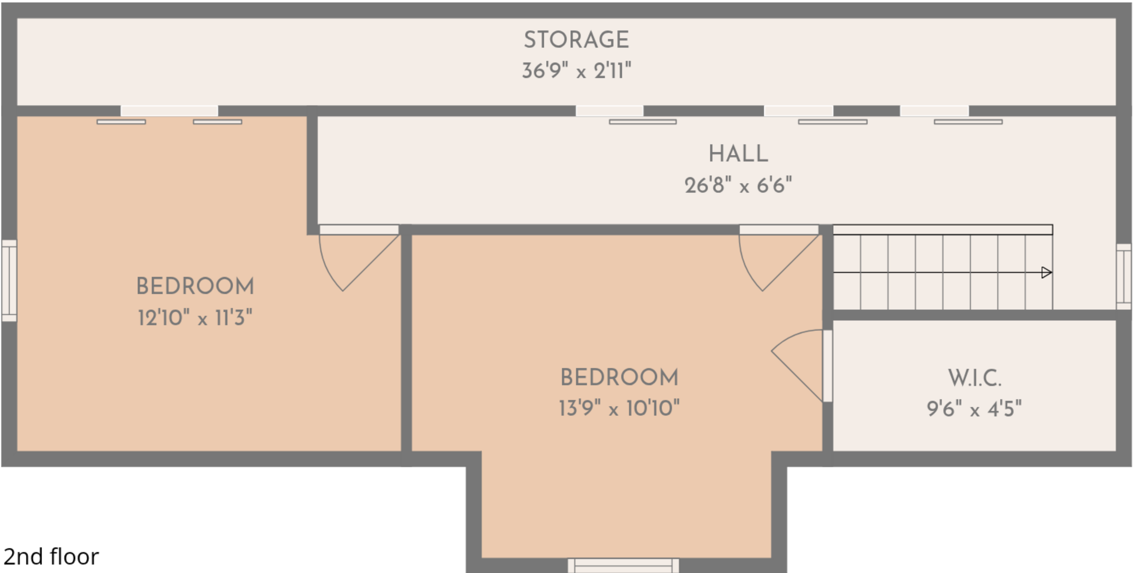
2nd floor
