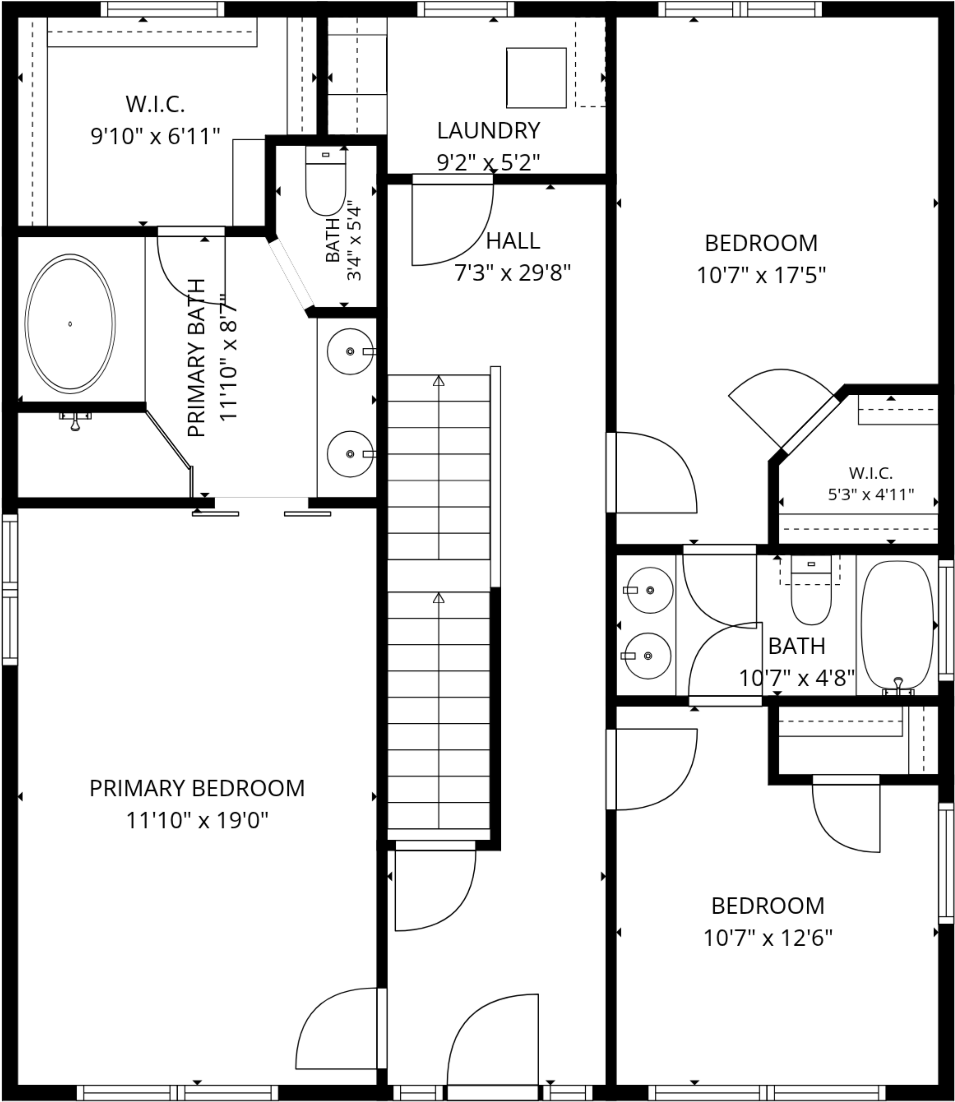
2nd floor
