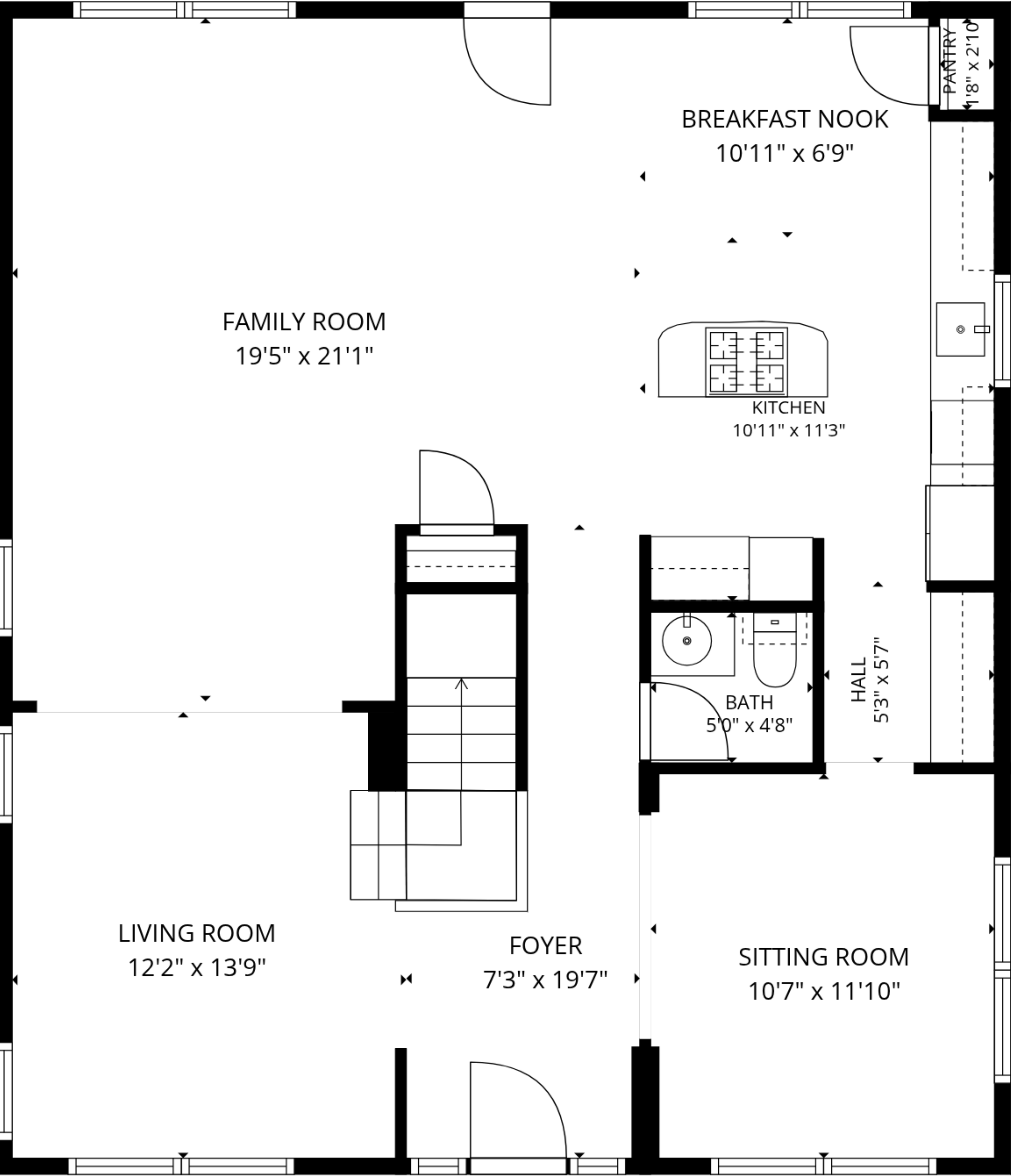
1st floor
