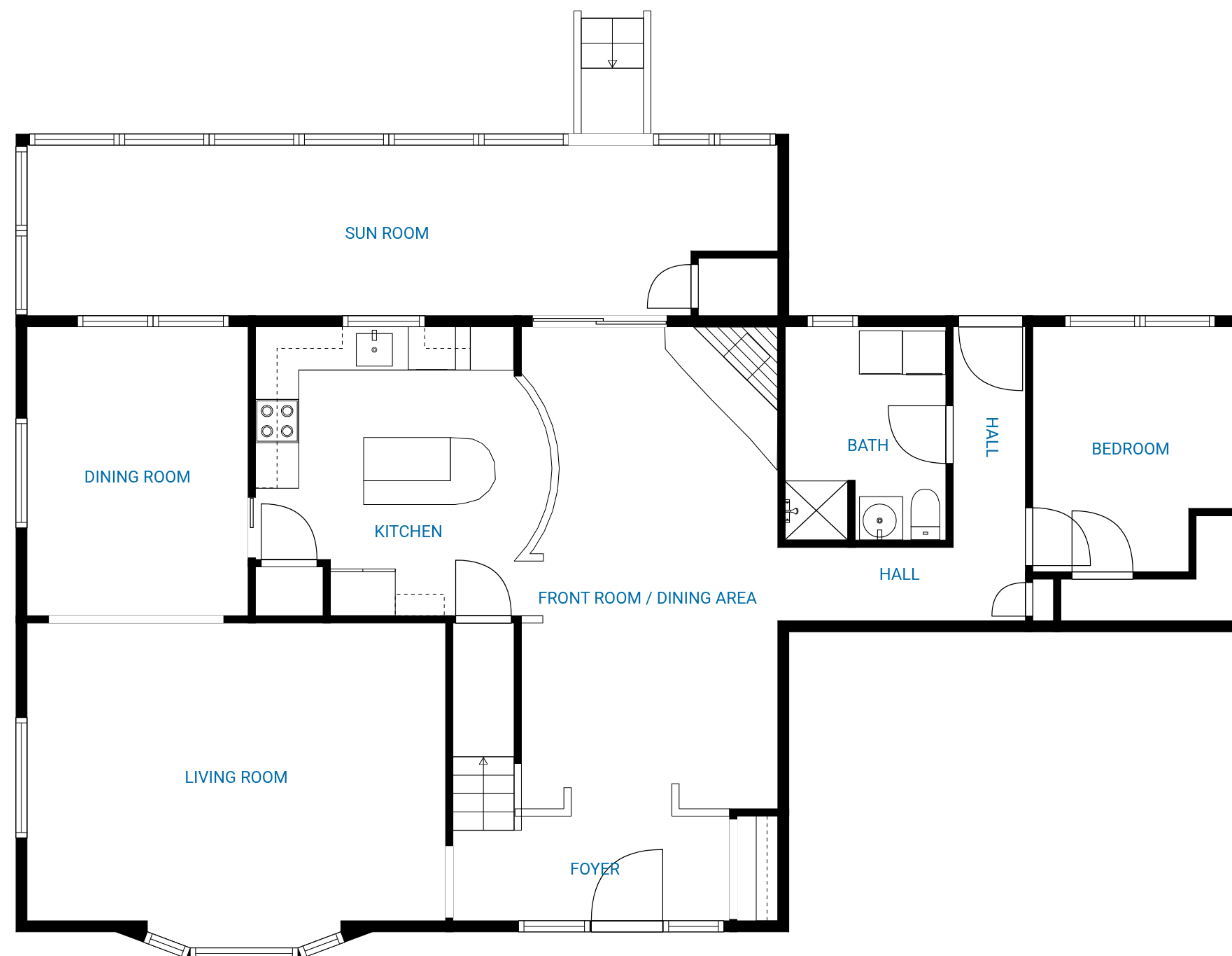
1st floor
