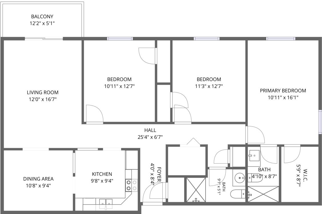
1st floor
