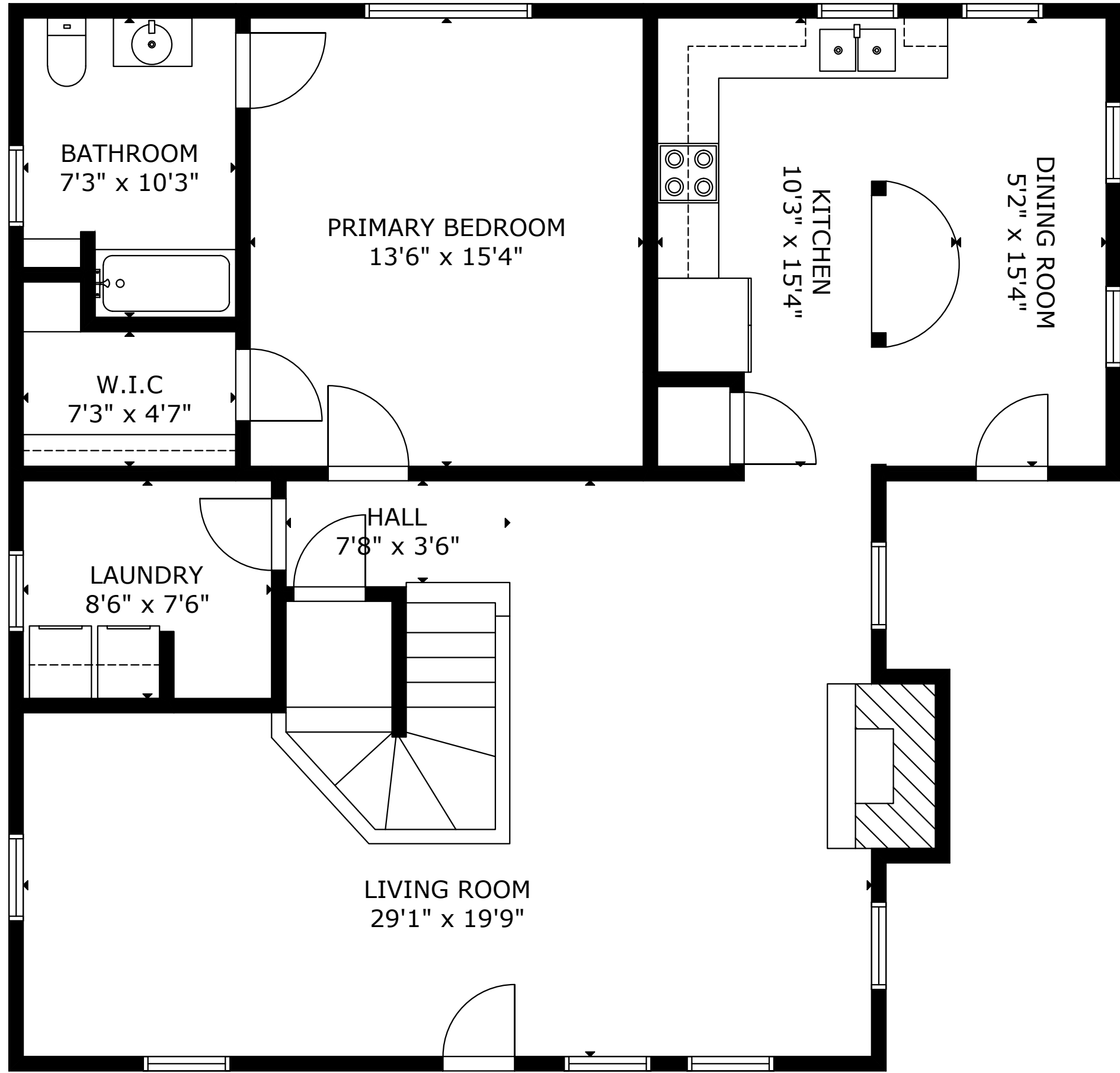
MAIN FLOOR
