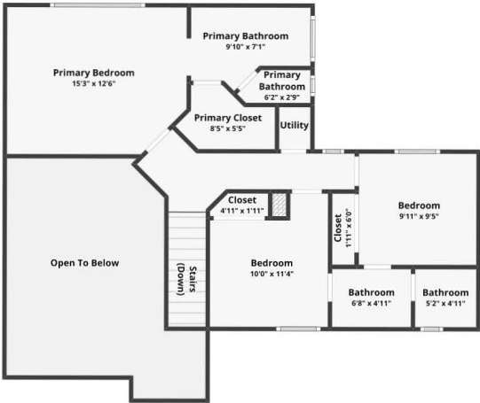
FLOOR 2 Finished area: ~662.89 sq. ft.
