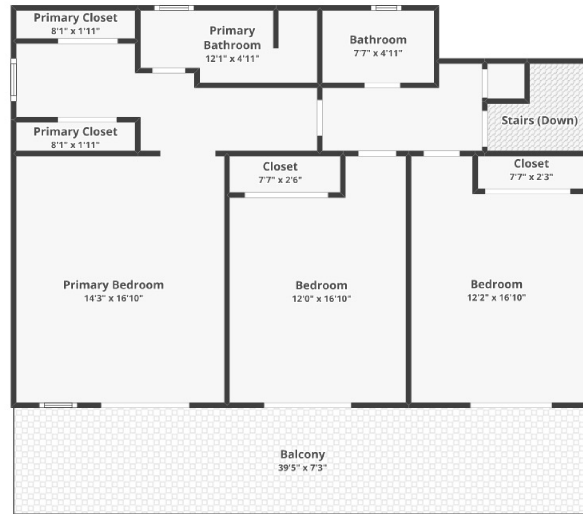
FLOOR 2
