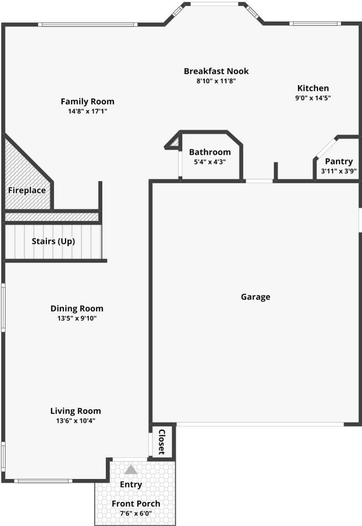
FLOOR 1 Finished area: ~785.93 sq. ft.
