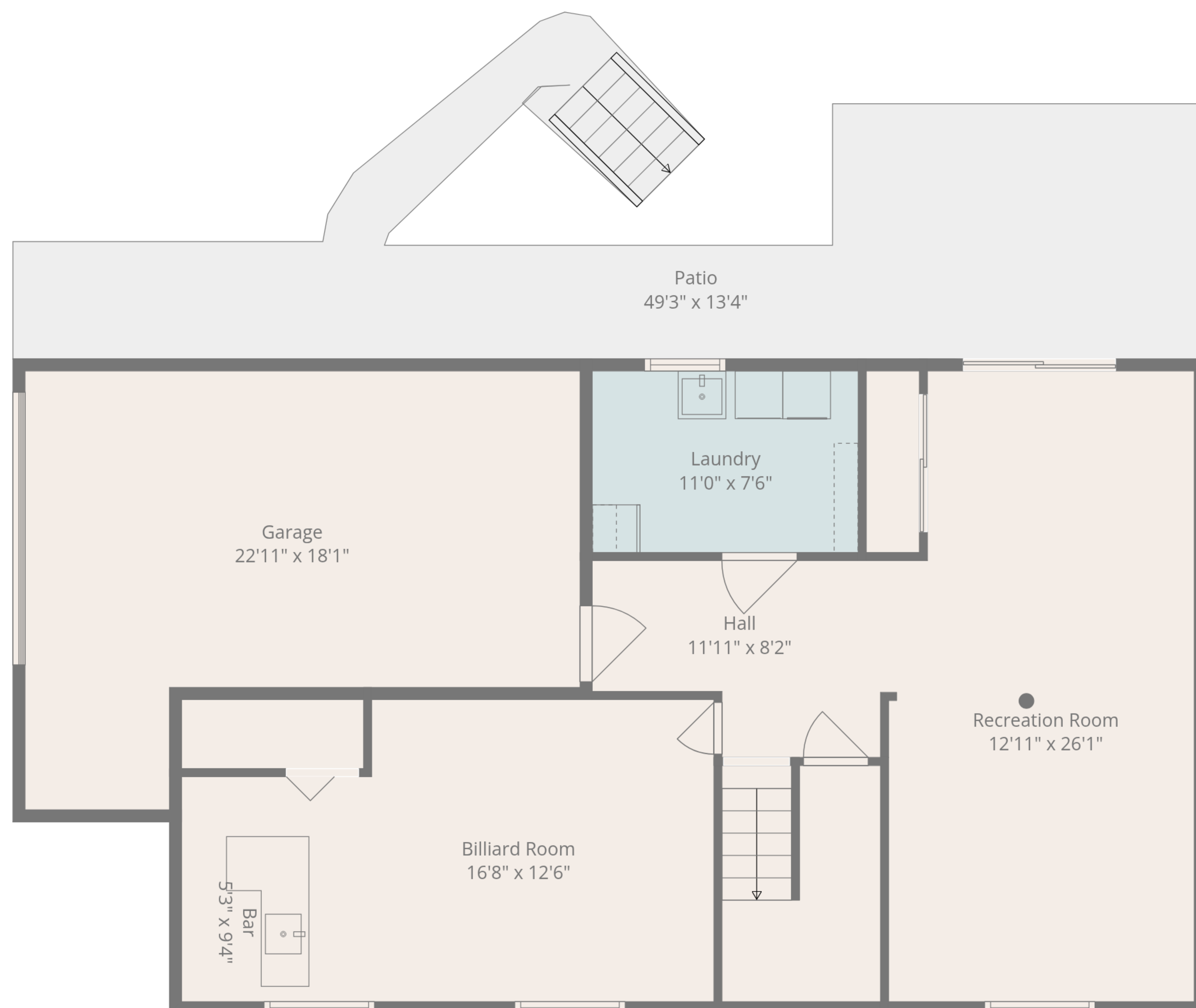
1st Floor
