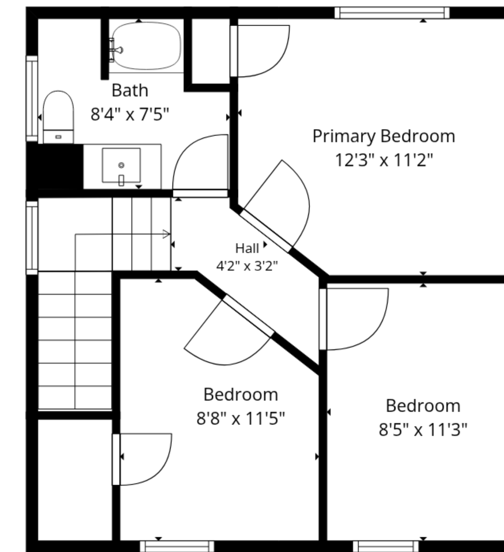
3rd Floor
