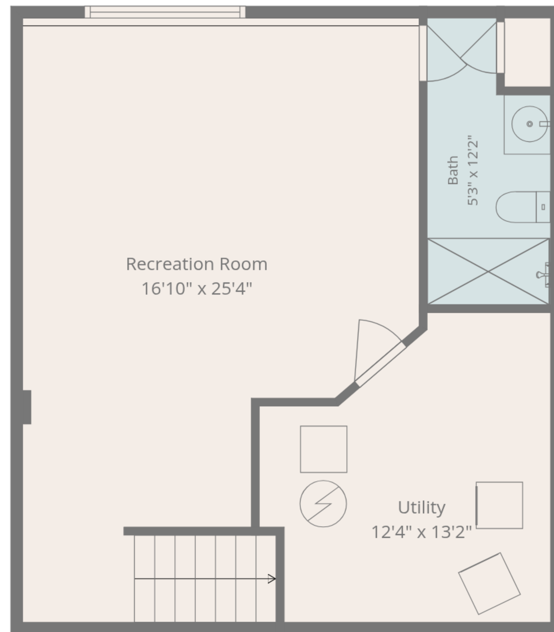
Basement
