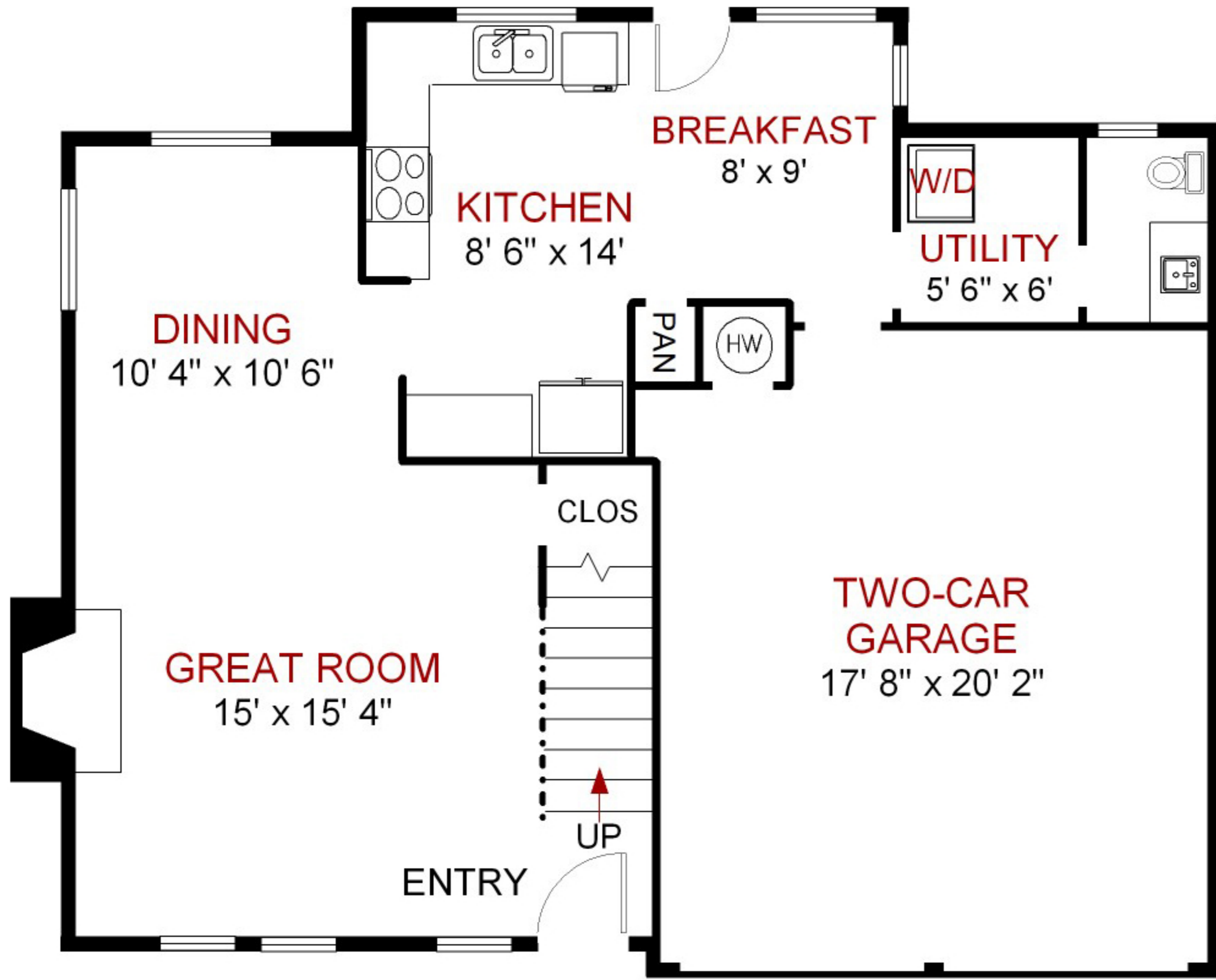
FIRST FLOOR
