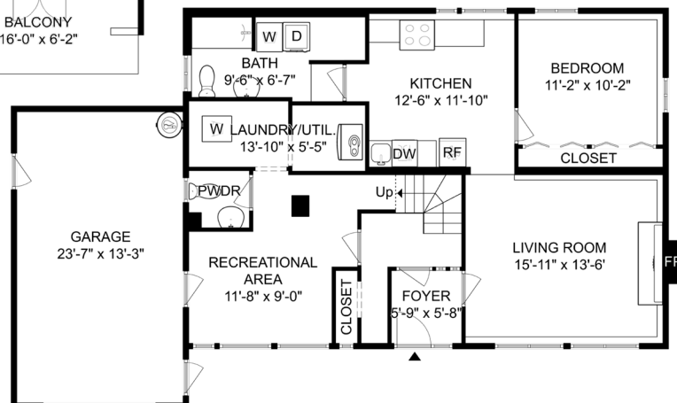
LOWER FLOOR 1,082 sq.ft. | Ceiling Height: 6'-3" to 7'-6"
