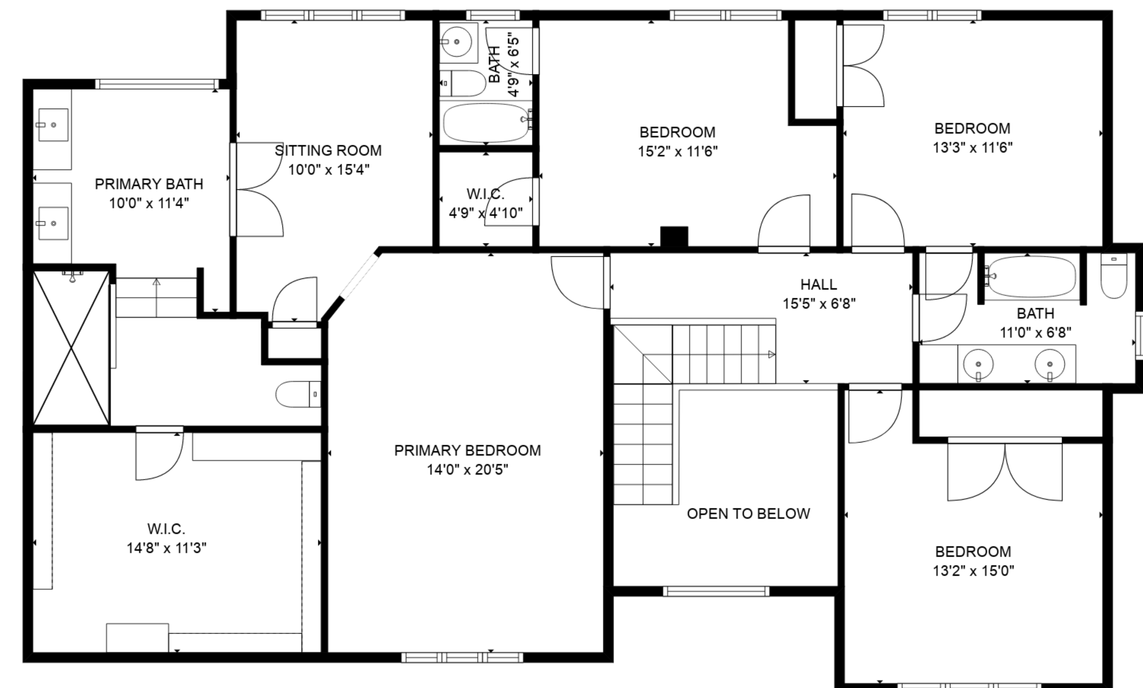
FLOOR 3
