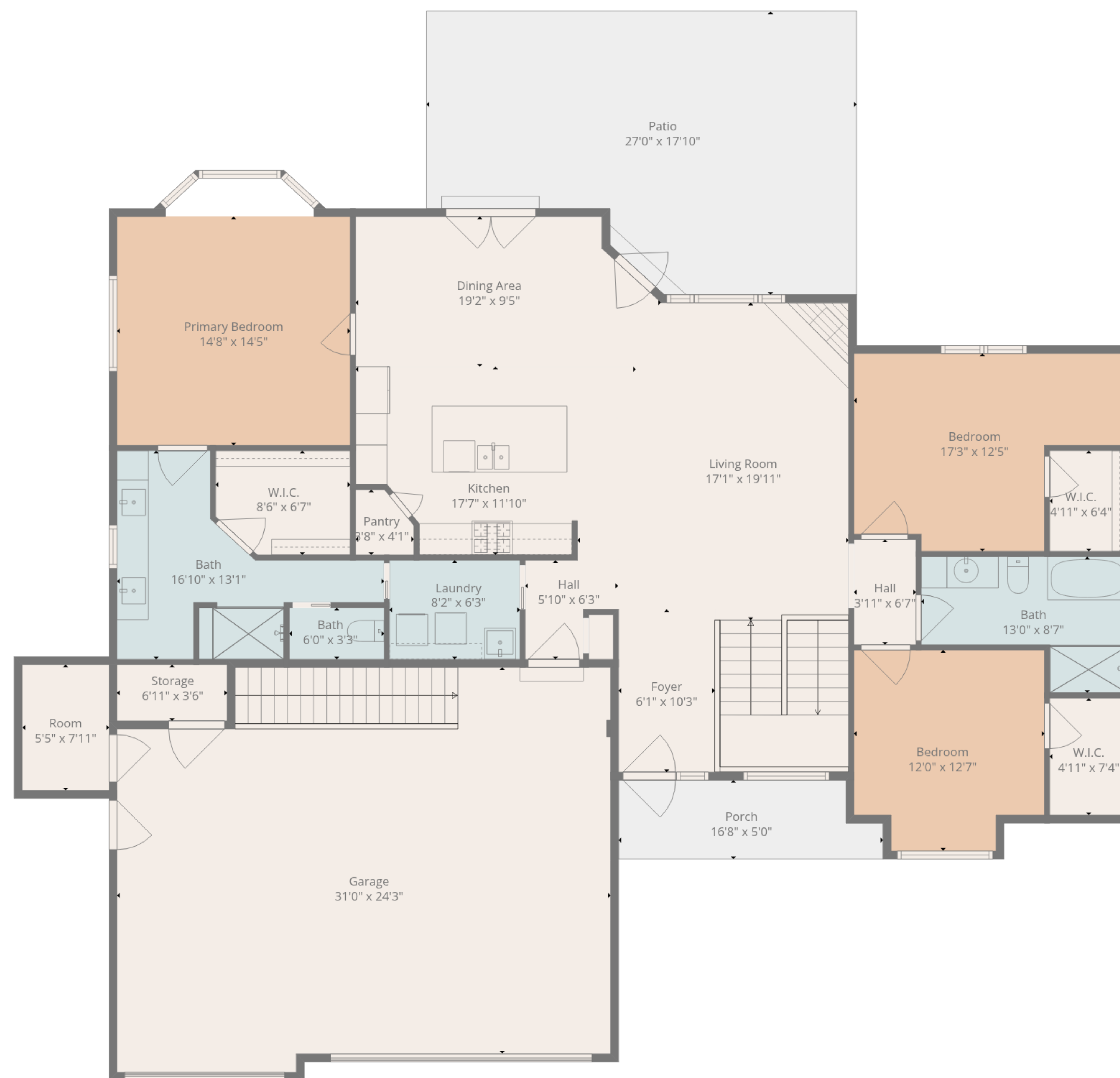
1st Floor
