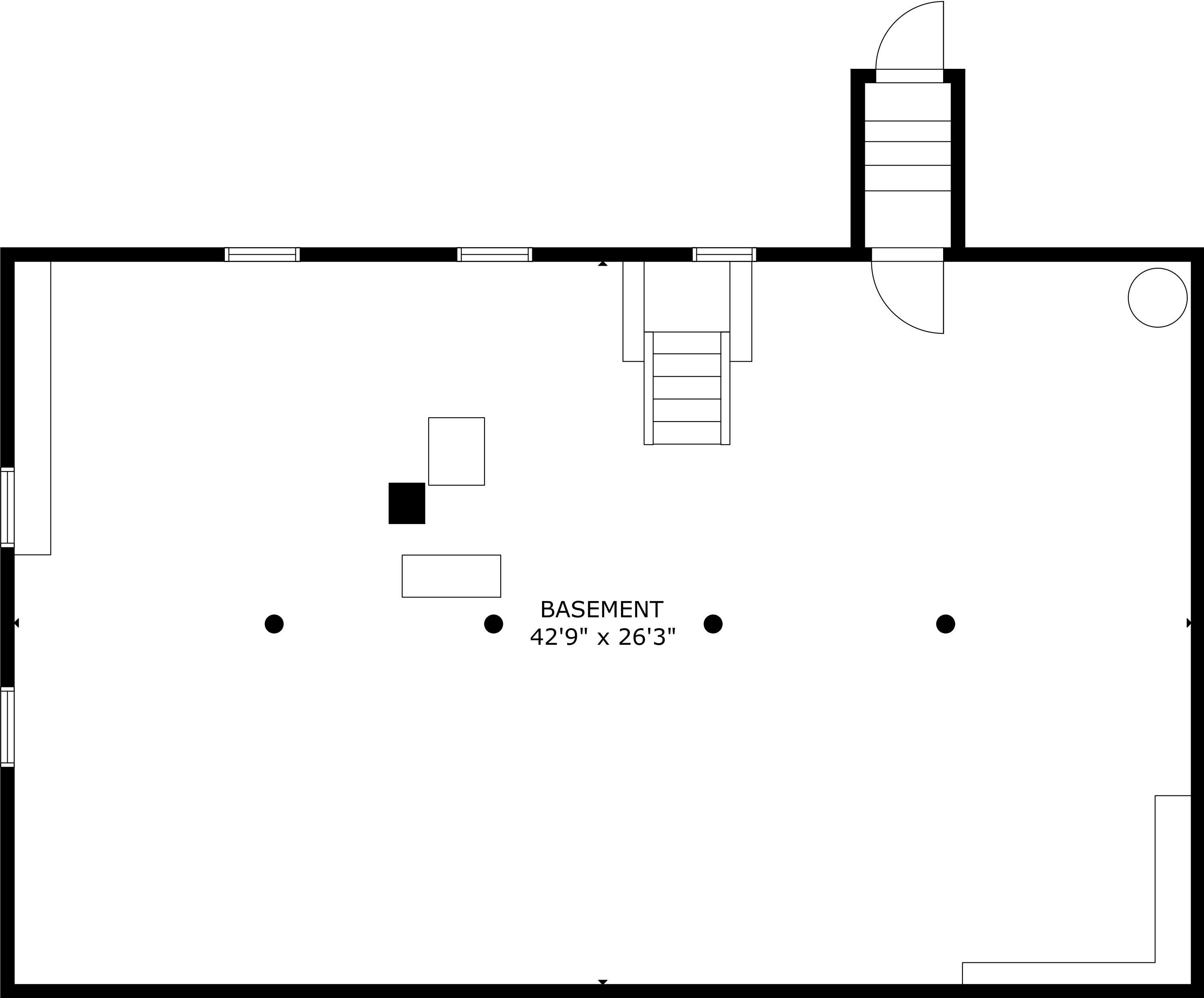
LOWER FLOOR
