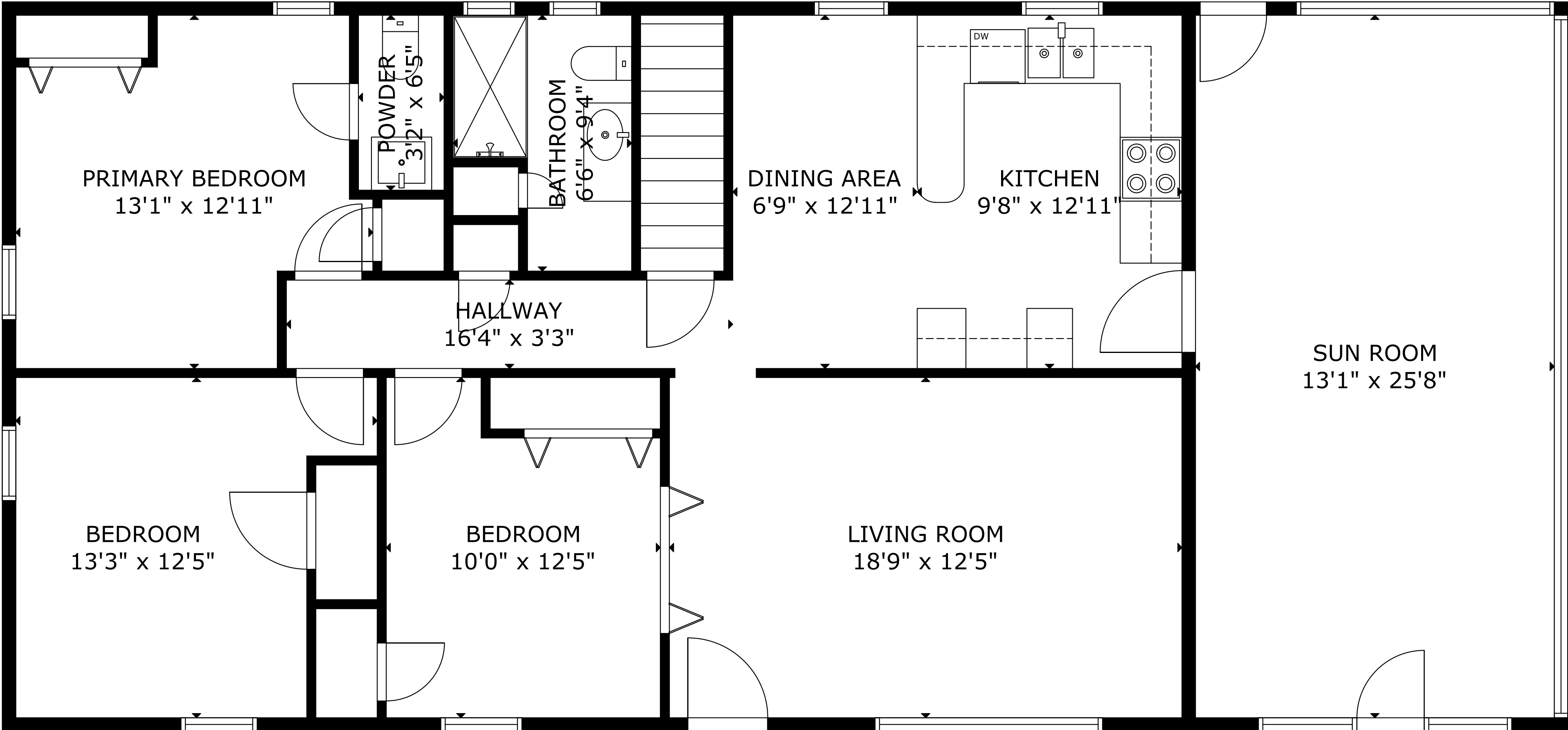
MAIN FLOOR
