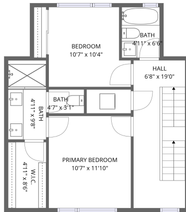
3rd floor
