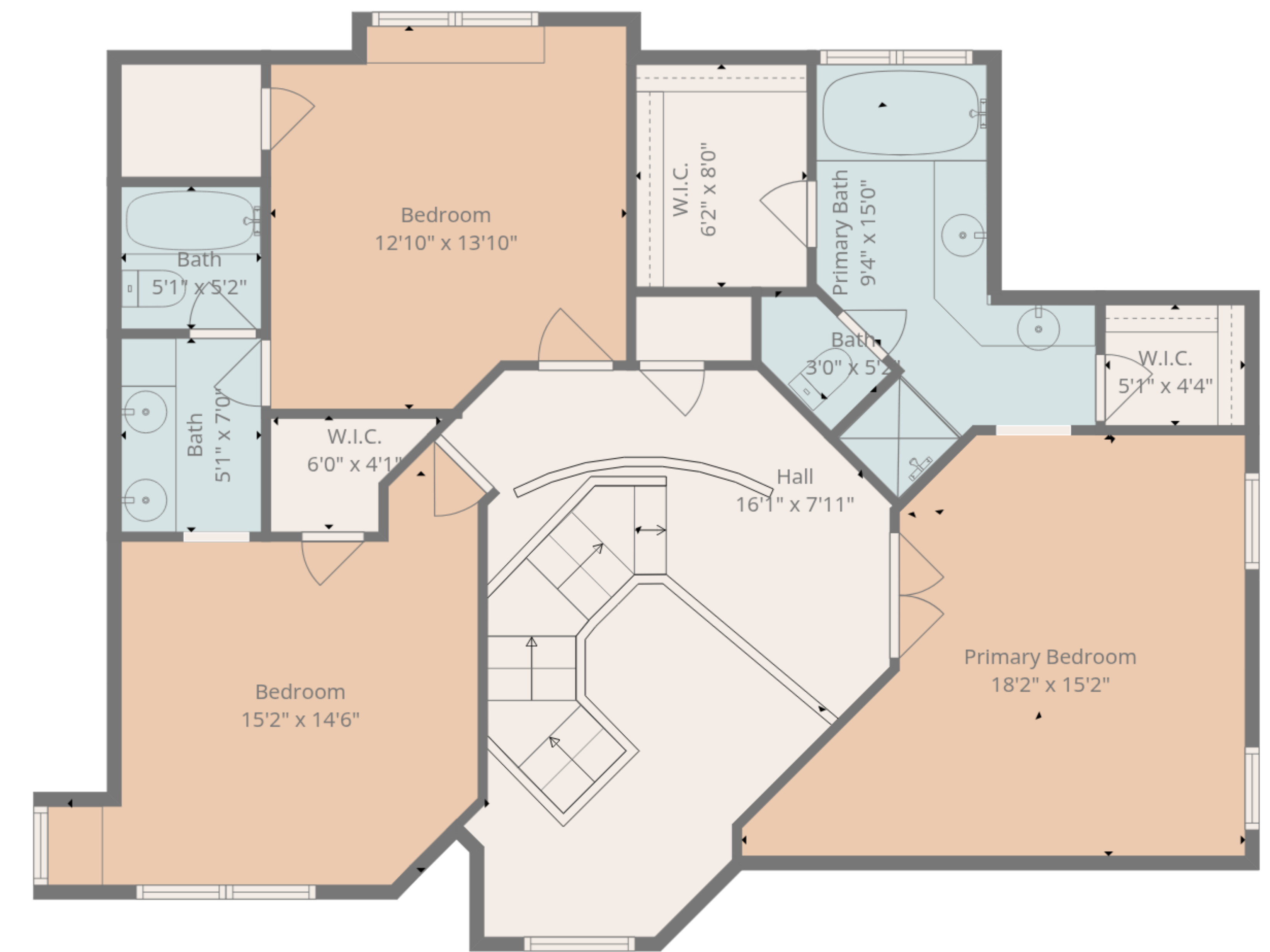
2nd Floor
