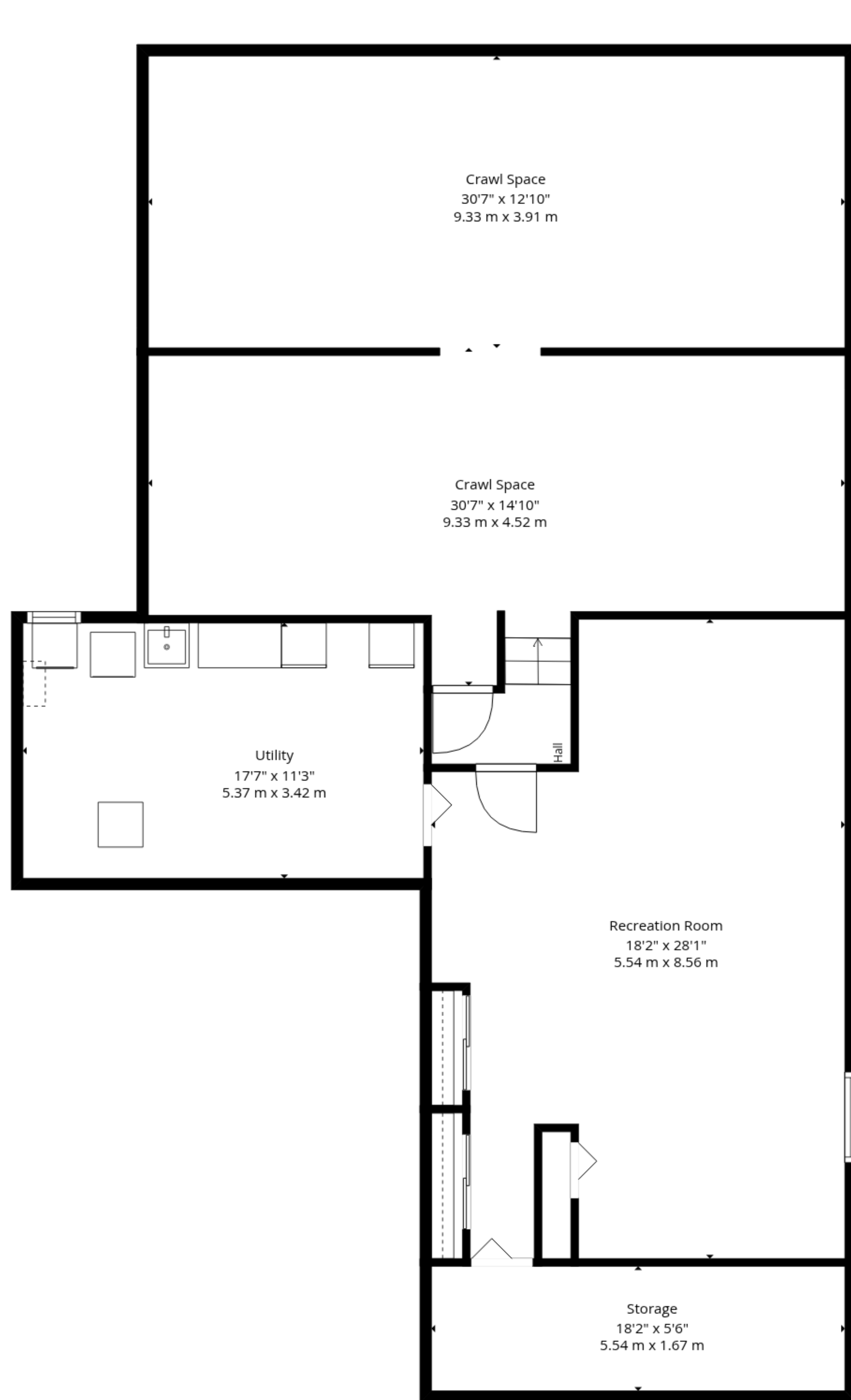
Basement
