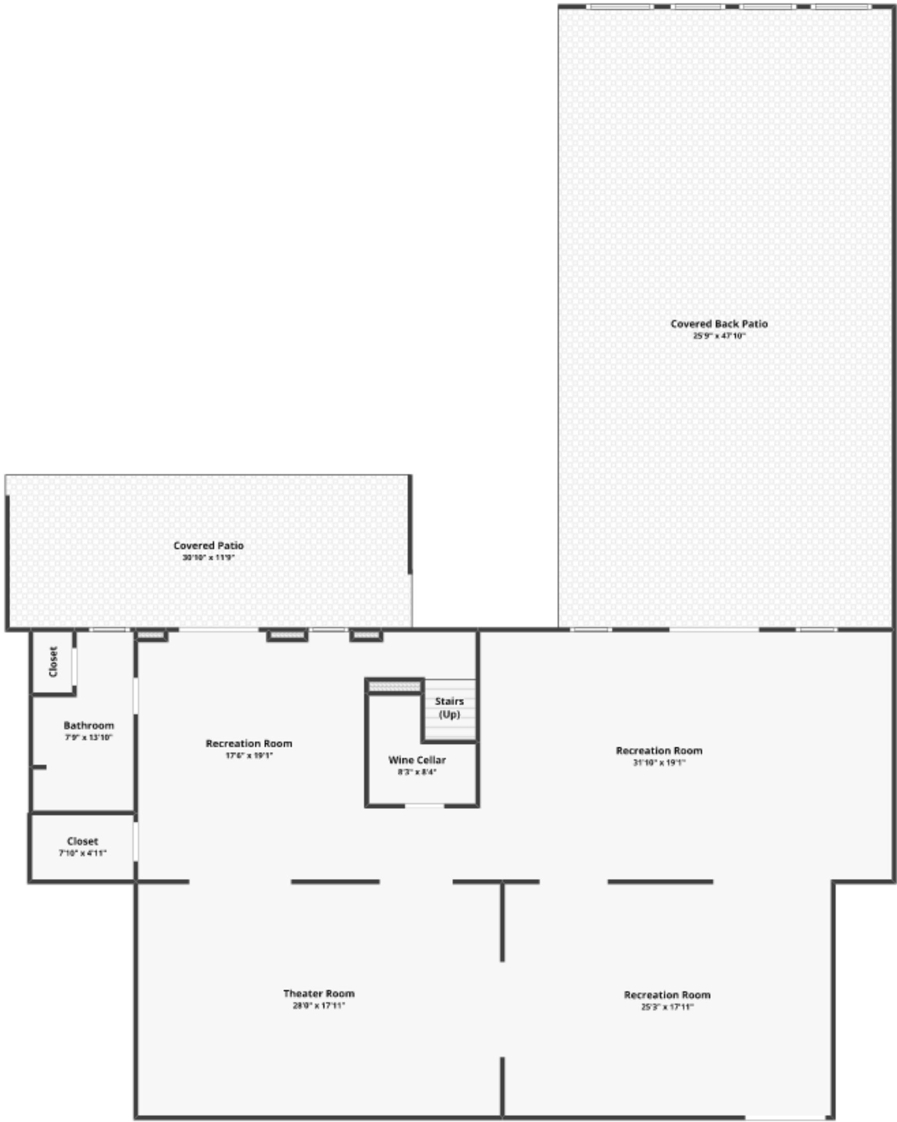
BASEMENT
