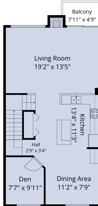
Main Floor
