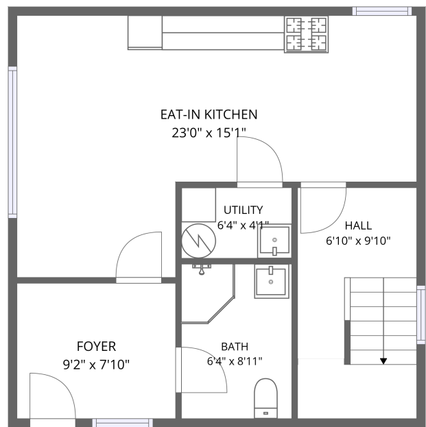
1st floor
