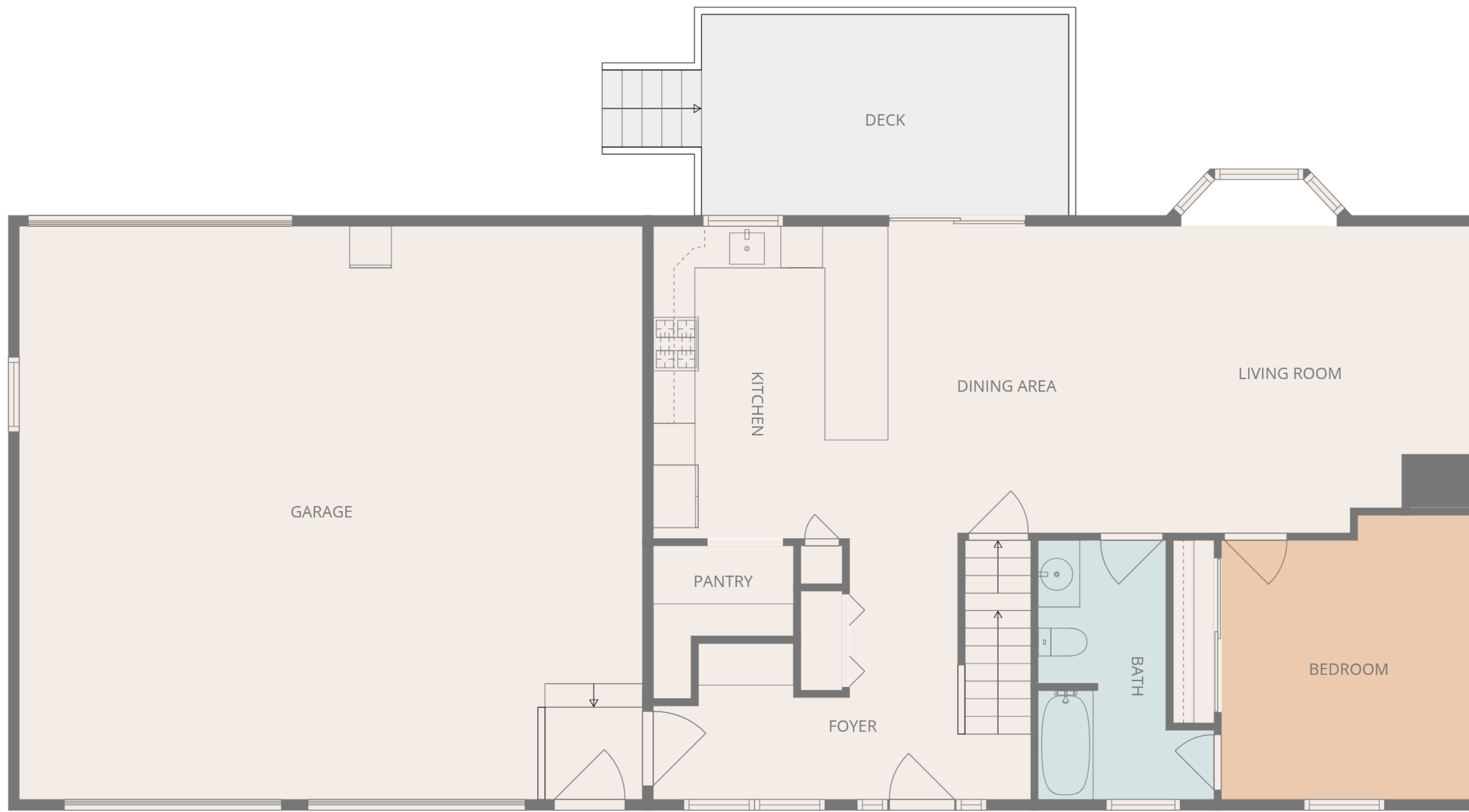
1st floor
