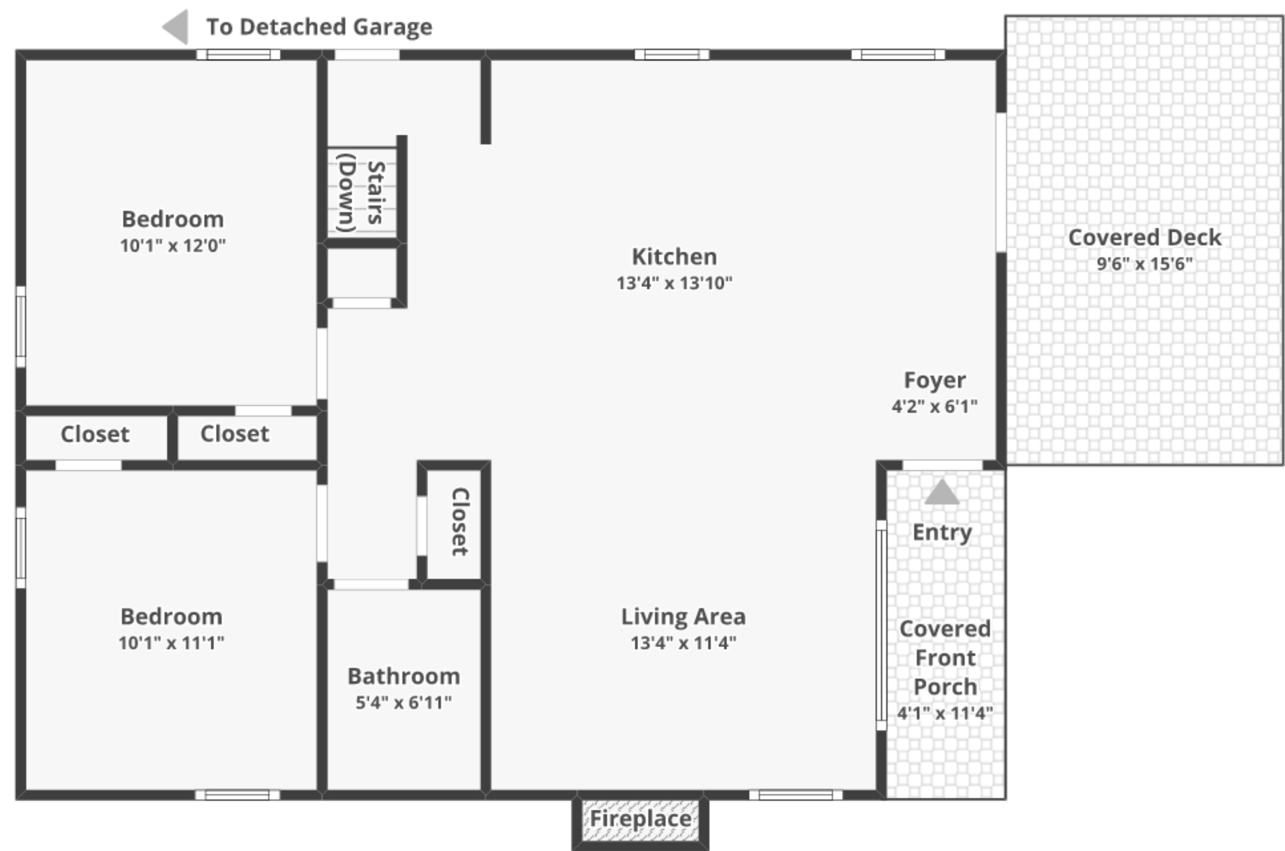
FLOOR 1
