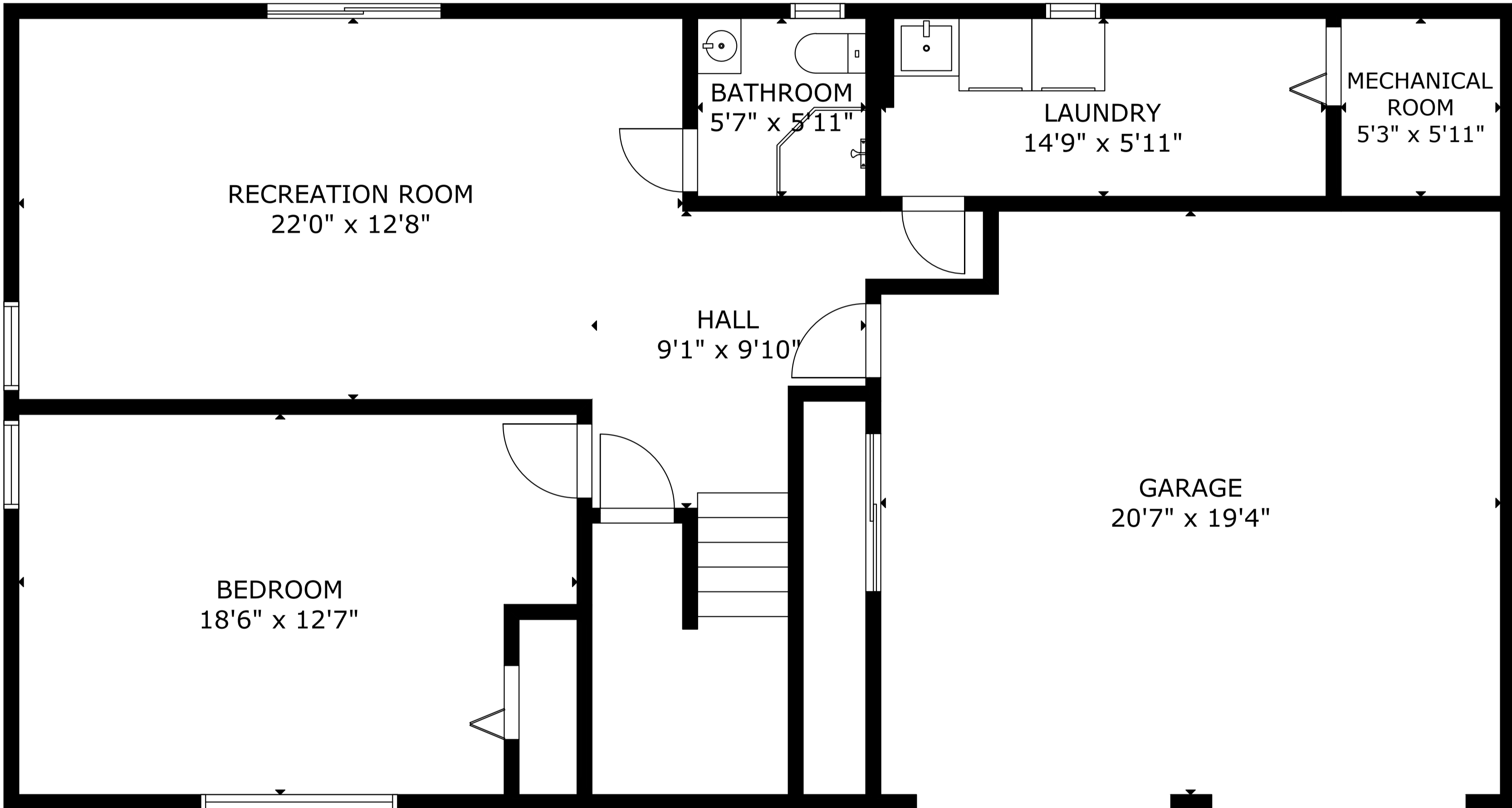
LOWER FLOOR
