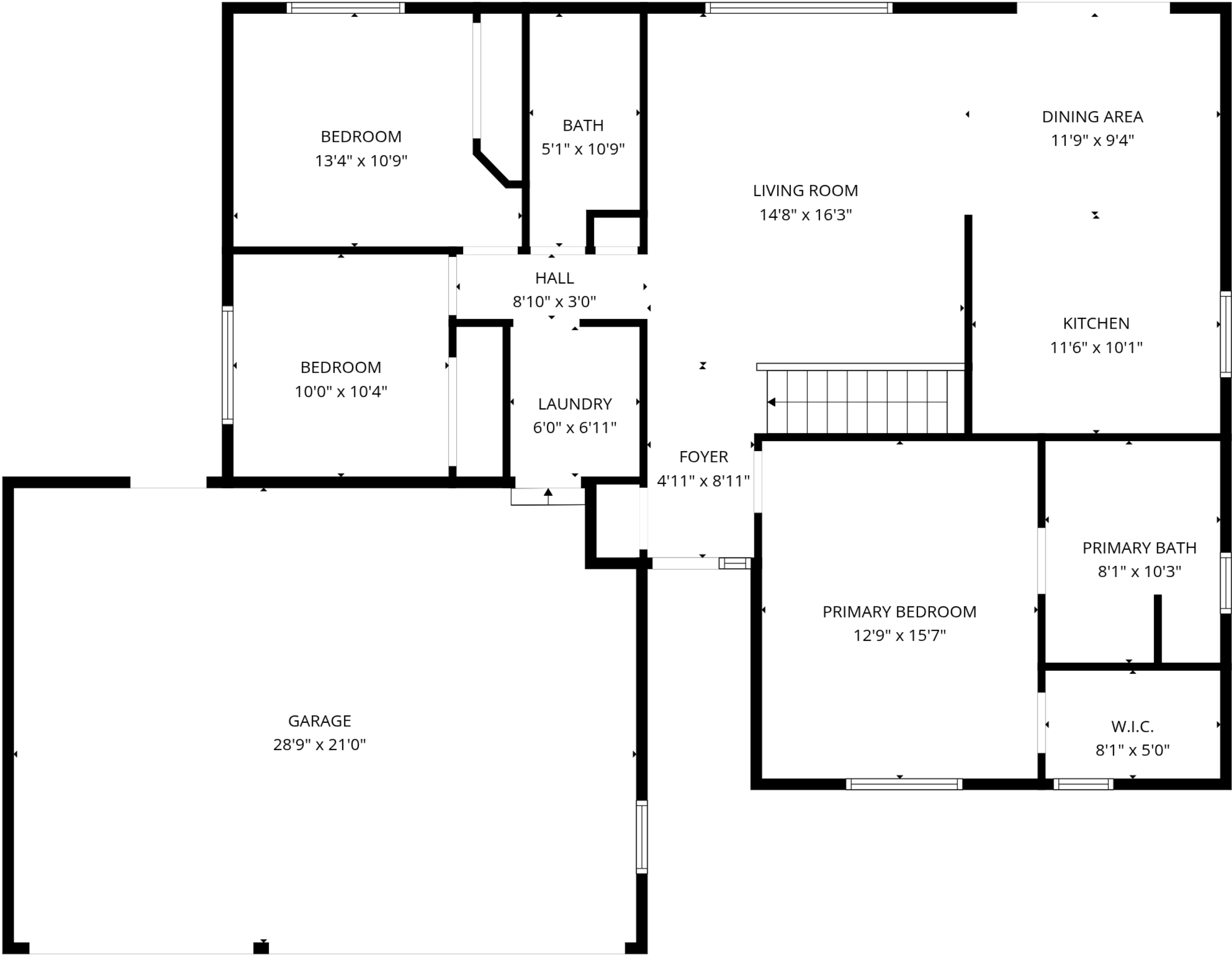
1st floor
