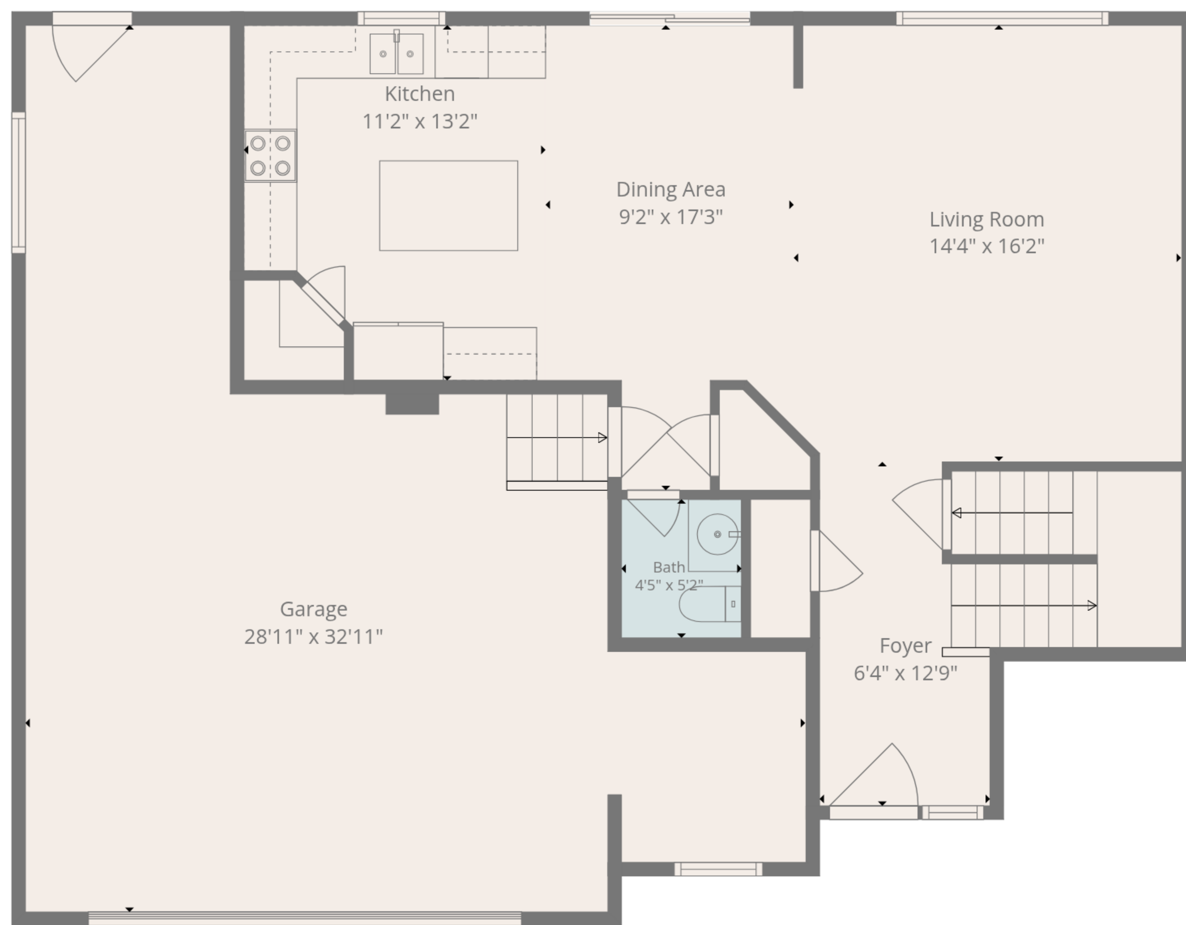
1st Floor
