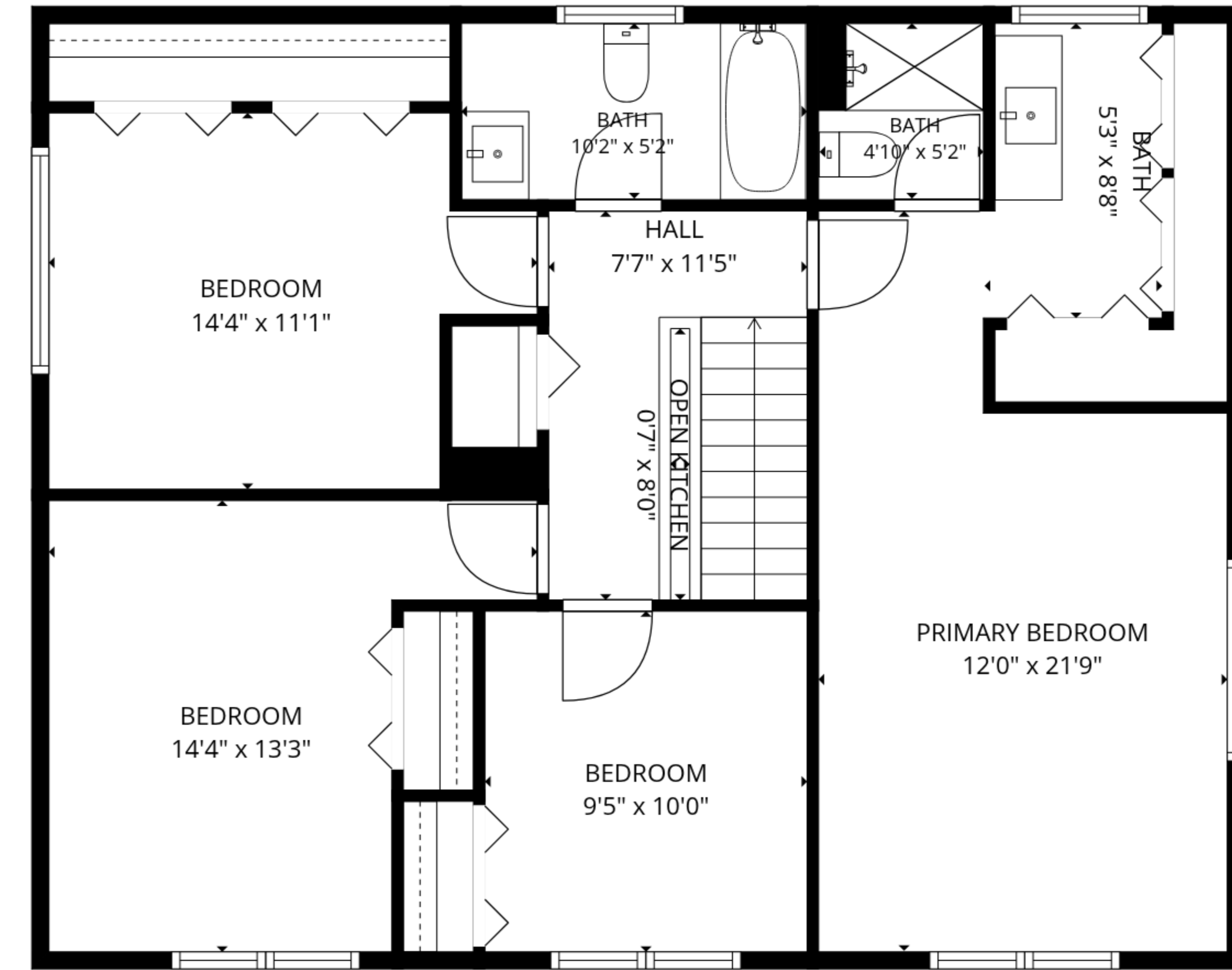
2nd floor
