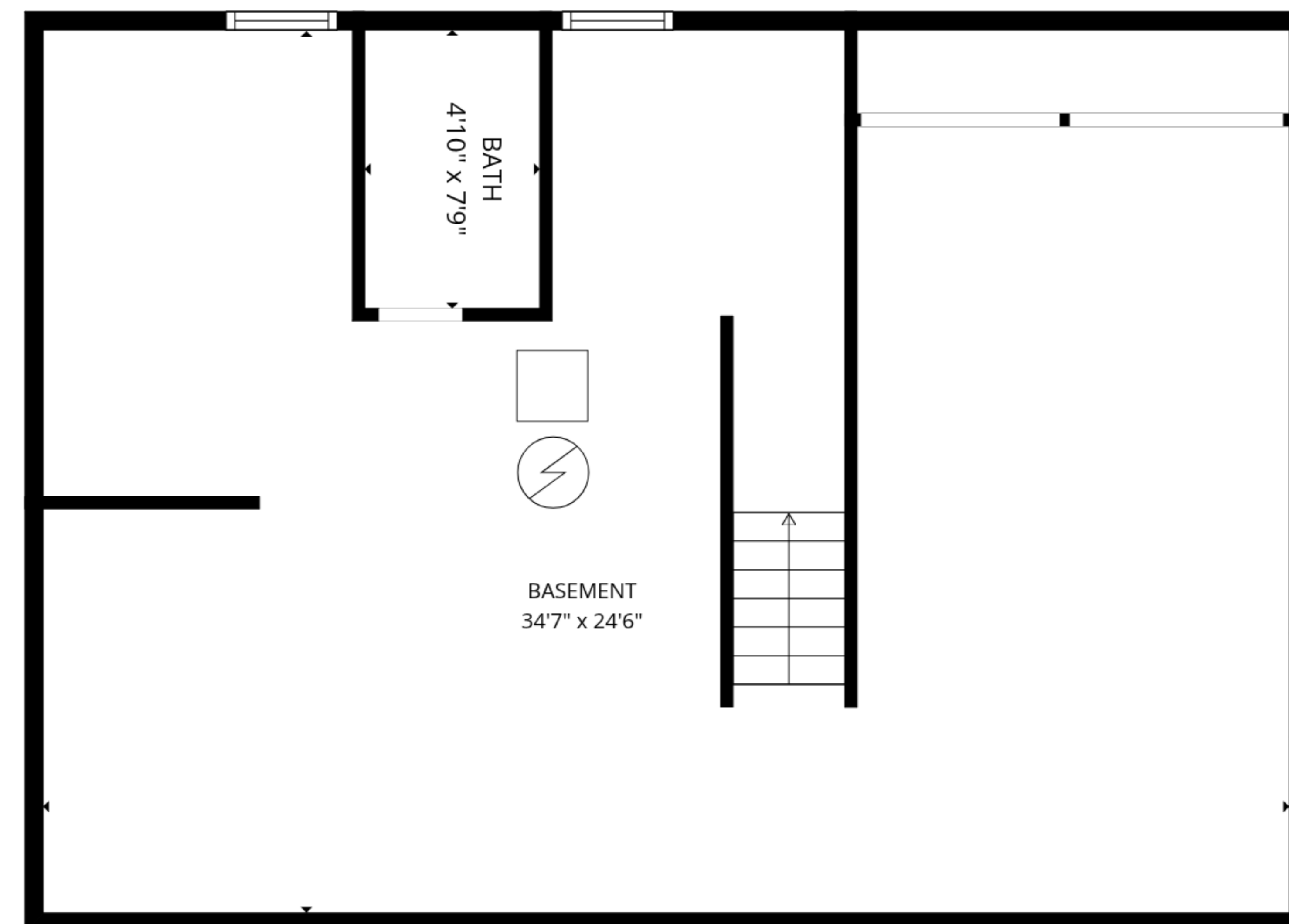
Basement
