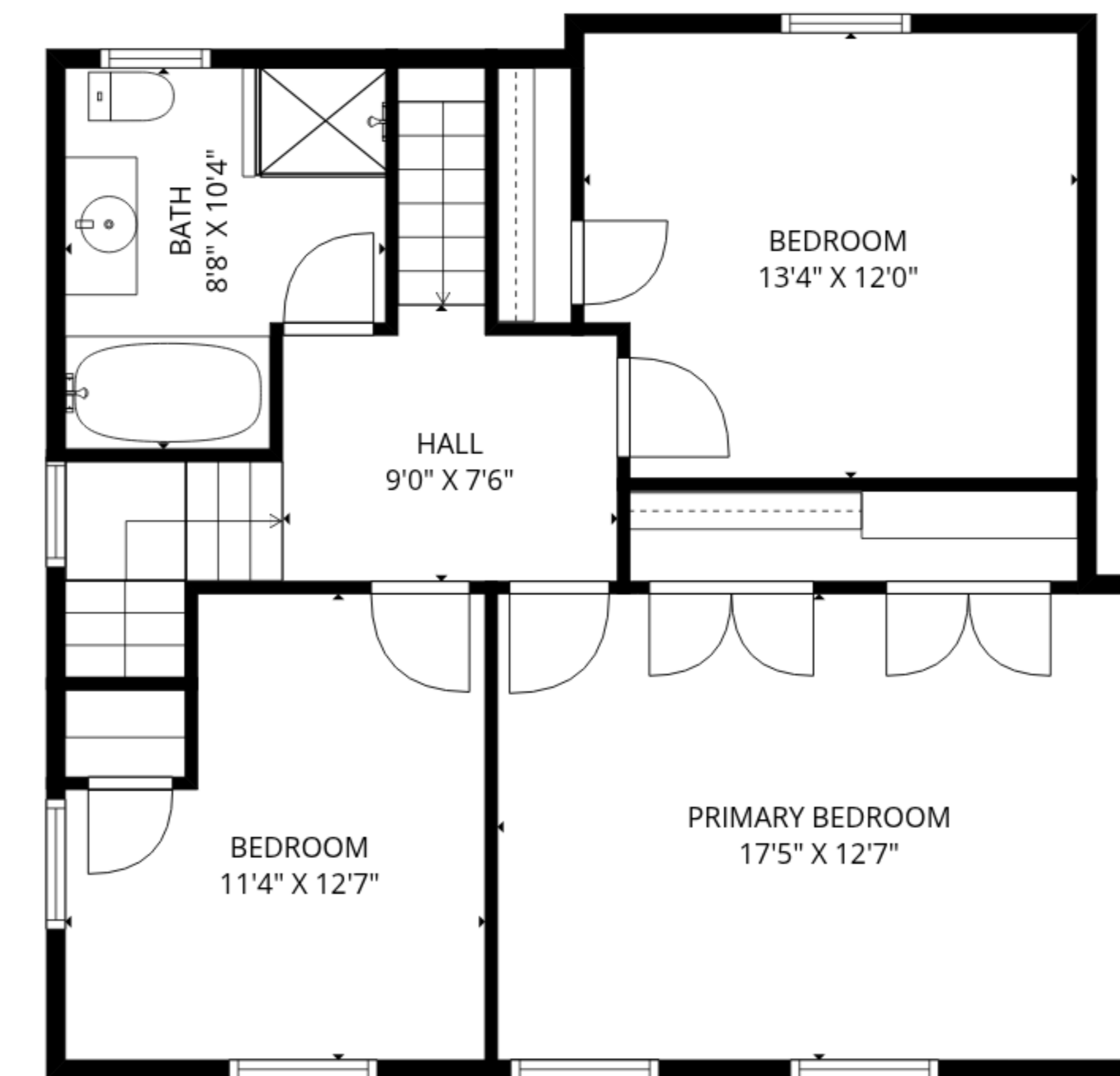
2ND FLOOR
