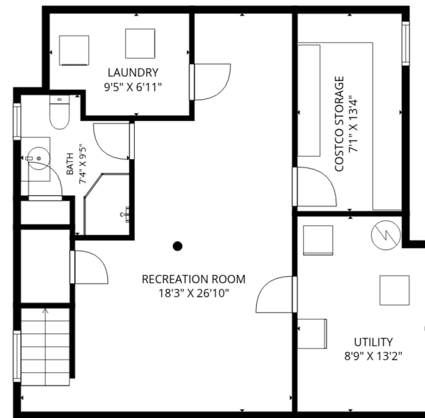
BASEMENT
